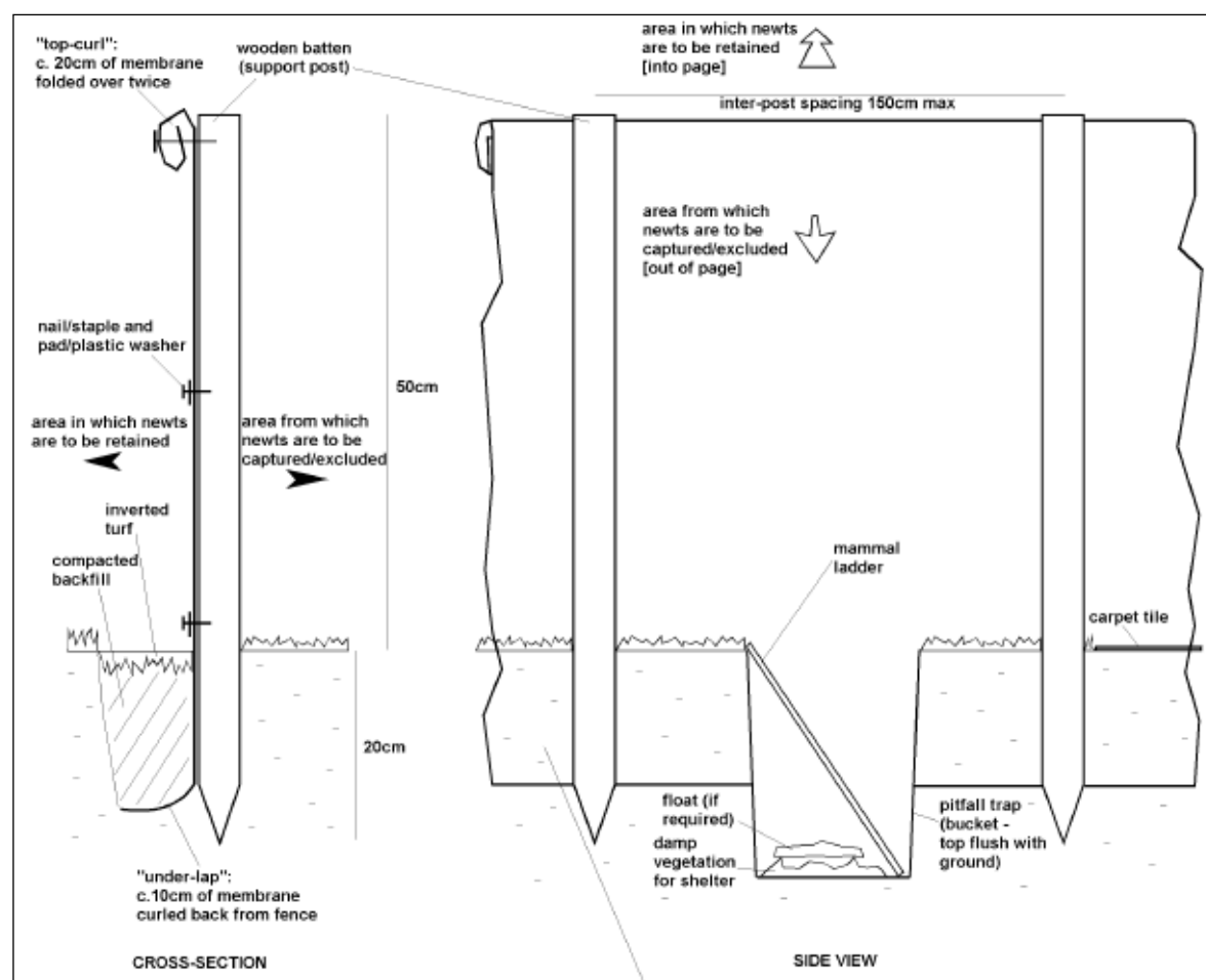
Drawing 1. Drift / Exclusion Fencing with Pitfall Trap Installation Specification
