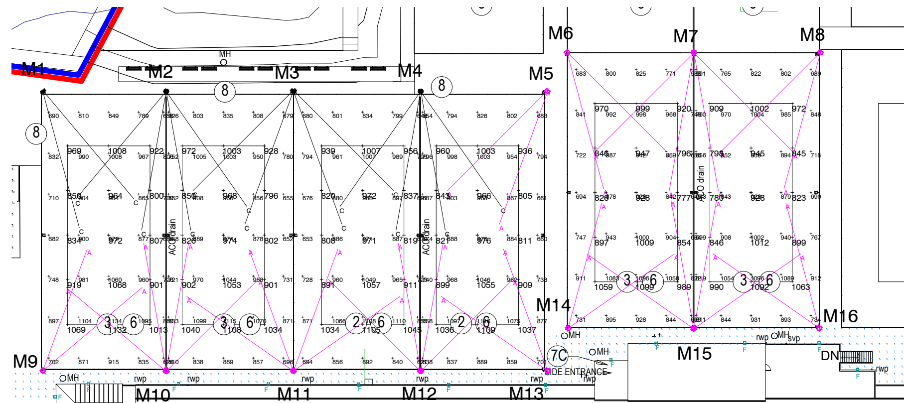
Tennis Court 3-8 TPA Horizontal Illuminance - Separately Switched
