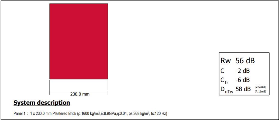
Figure 4 - INSUL prediction of sound insulation of proposed separating wall construction The predictions indicate that the wall construction is likely to meet the recommended 57dB D_{nTw} performance.
