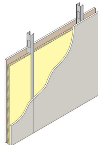
Figure 7 - Recommended internal wall constructions
