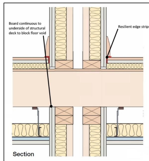
Figure 6 – Section detail illustrating how the separating floor should be junctioned with the separating walls
