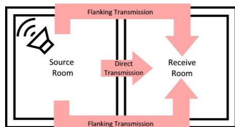
Figure 5 - Illustrating the difference between sound transmitted directly through a common area and flanking transmission
