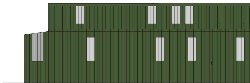
A 17 Side East 1:100
