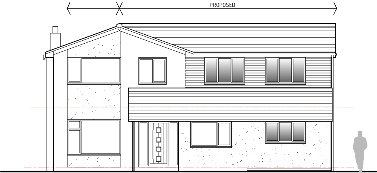
Front elevation 1:100
