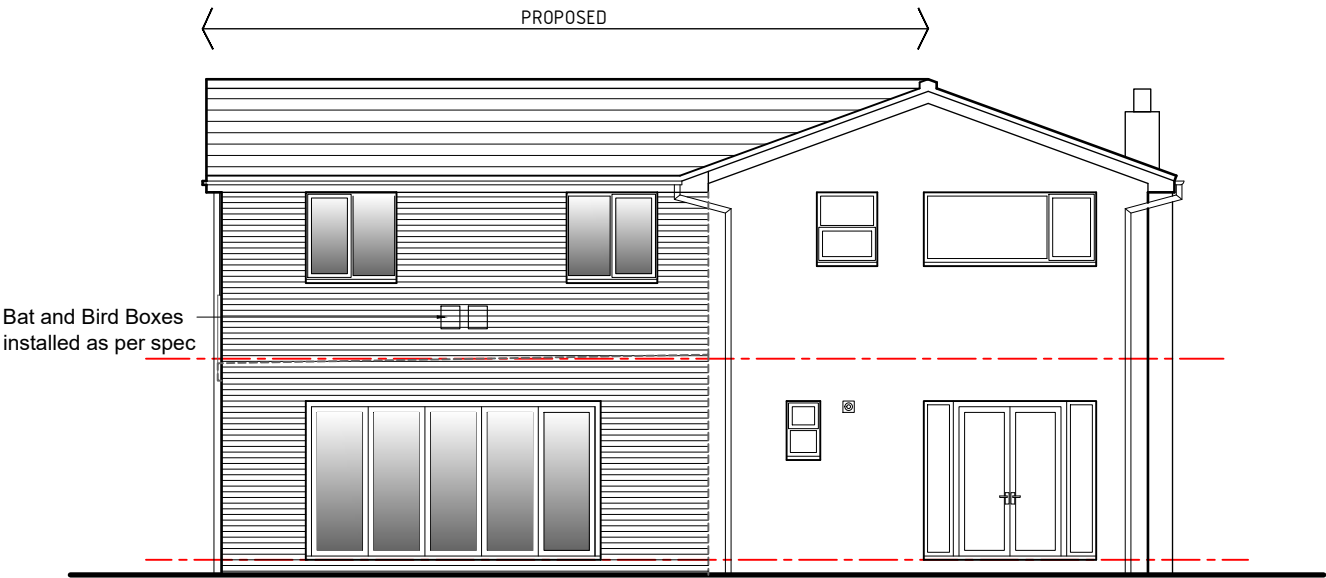
Rear elevation 1:100
