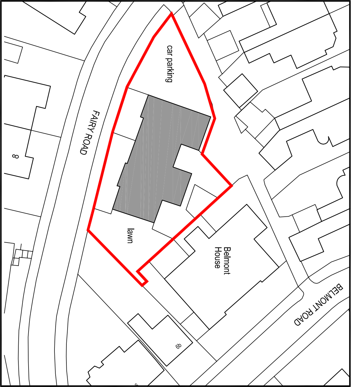
EXISTING site plan 1 to 500
