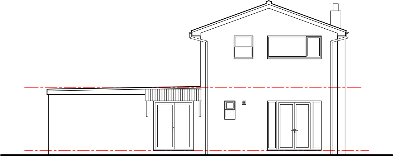
Rear elevation 1:100
