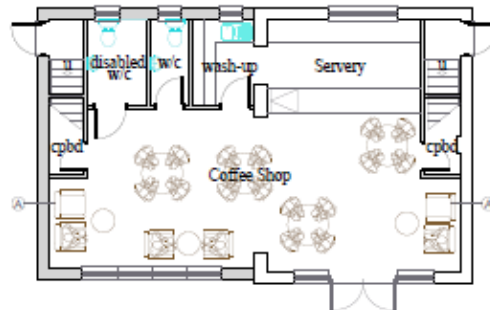
Ground Floor Plan 1:50 - Coffee Shop
