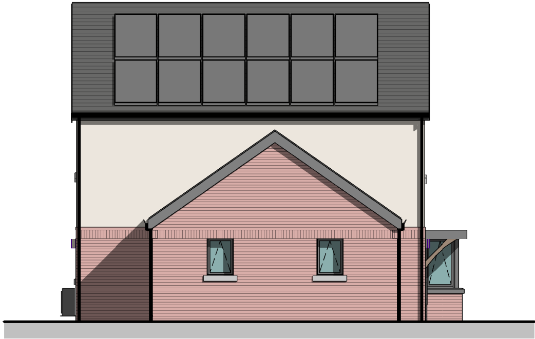
SIDE ELEVATIONa 1 : 100
