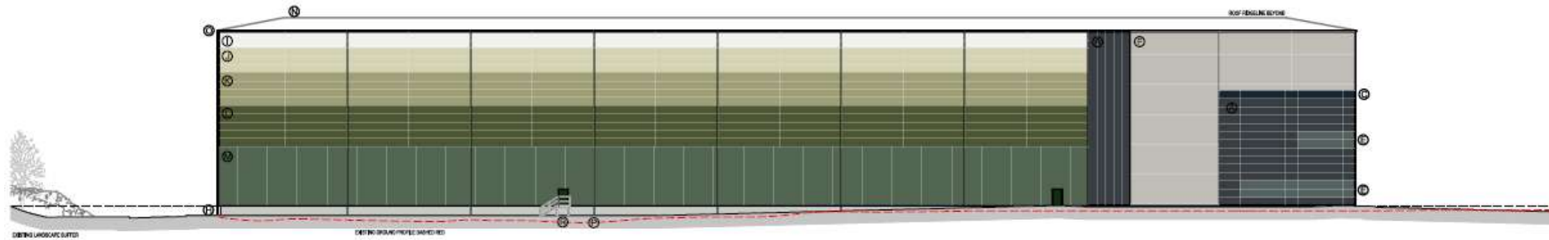
PROPOSED SOUTH WEST ELEVATION
