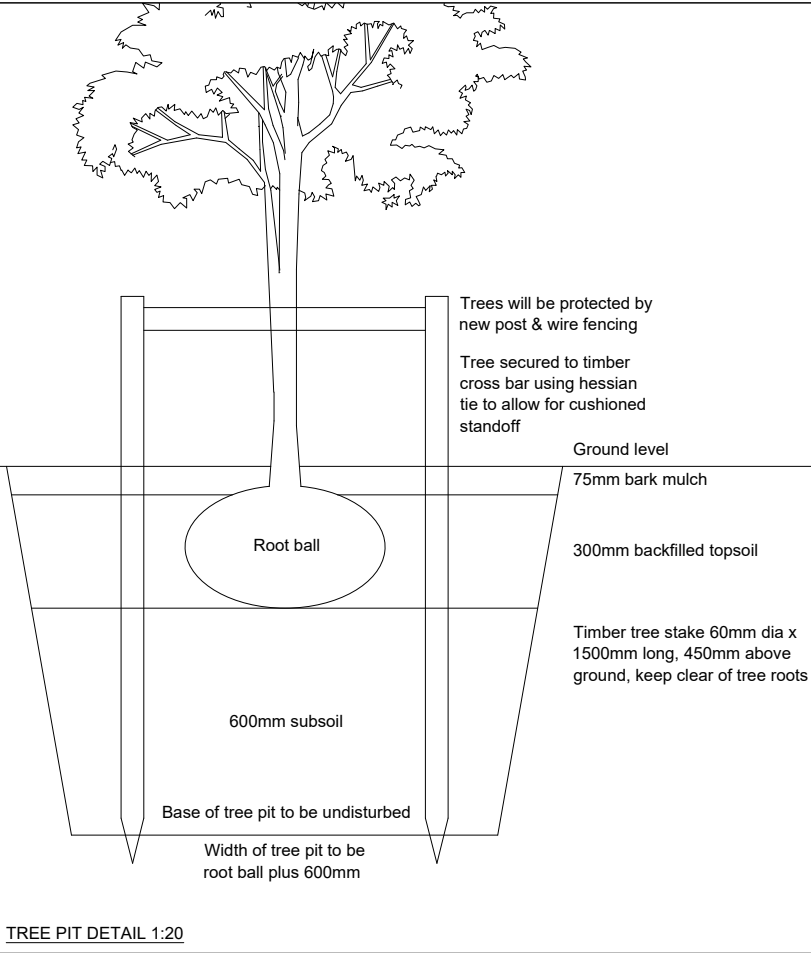
TREE PIT DETAIL 1:20
