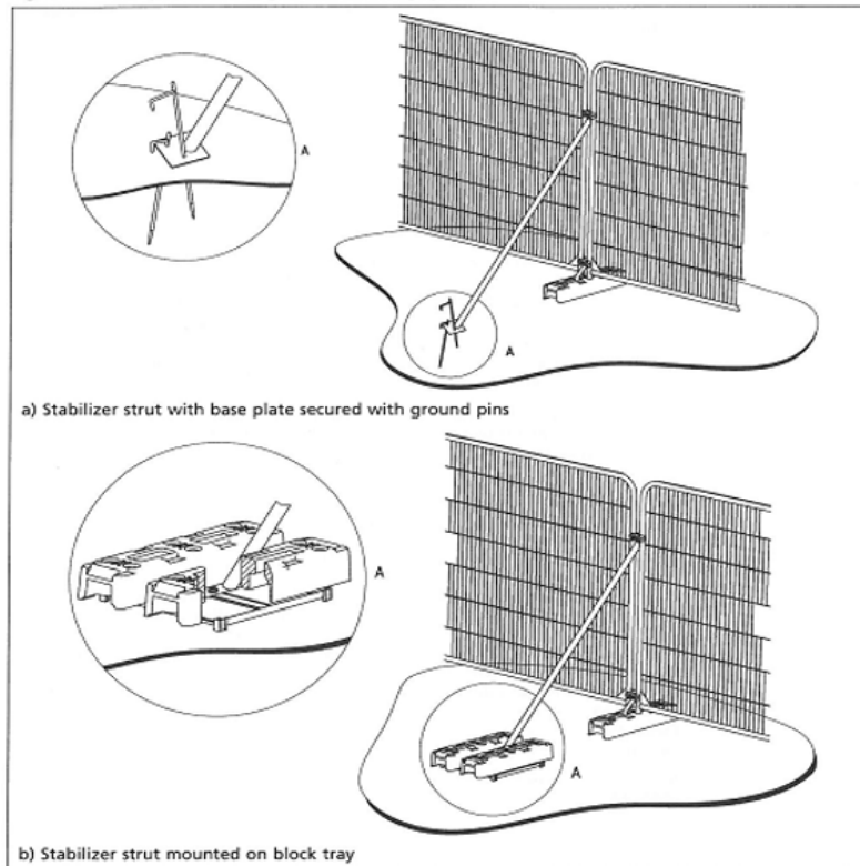
Figure 3 Examples of above-ground stabilizing systems
