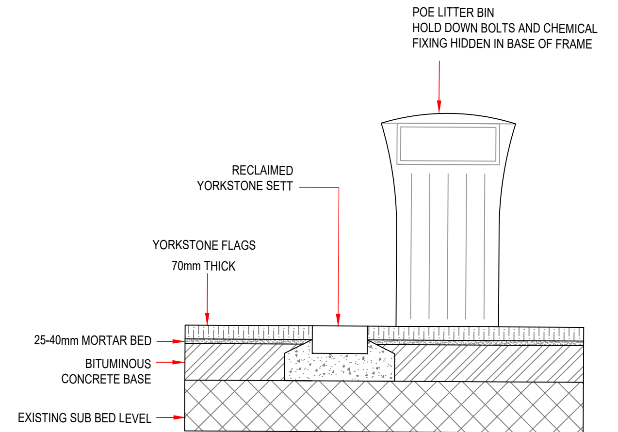
19 1:20 PRIMARY PEDESTRIAN ACCESS INTO MUSEUM / LITTER BIN
