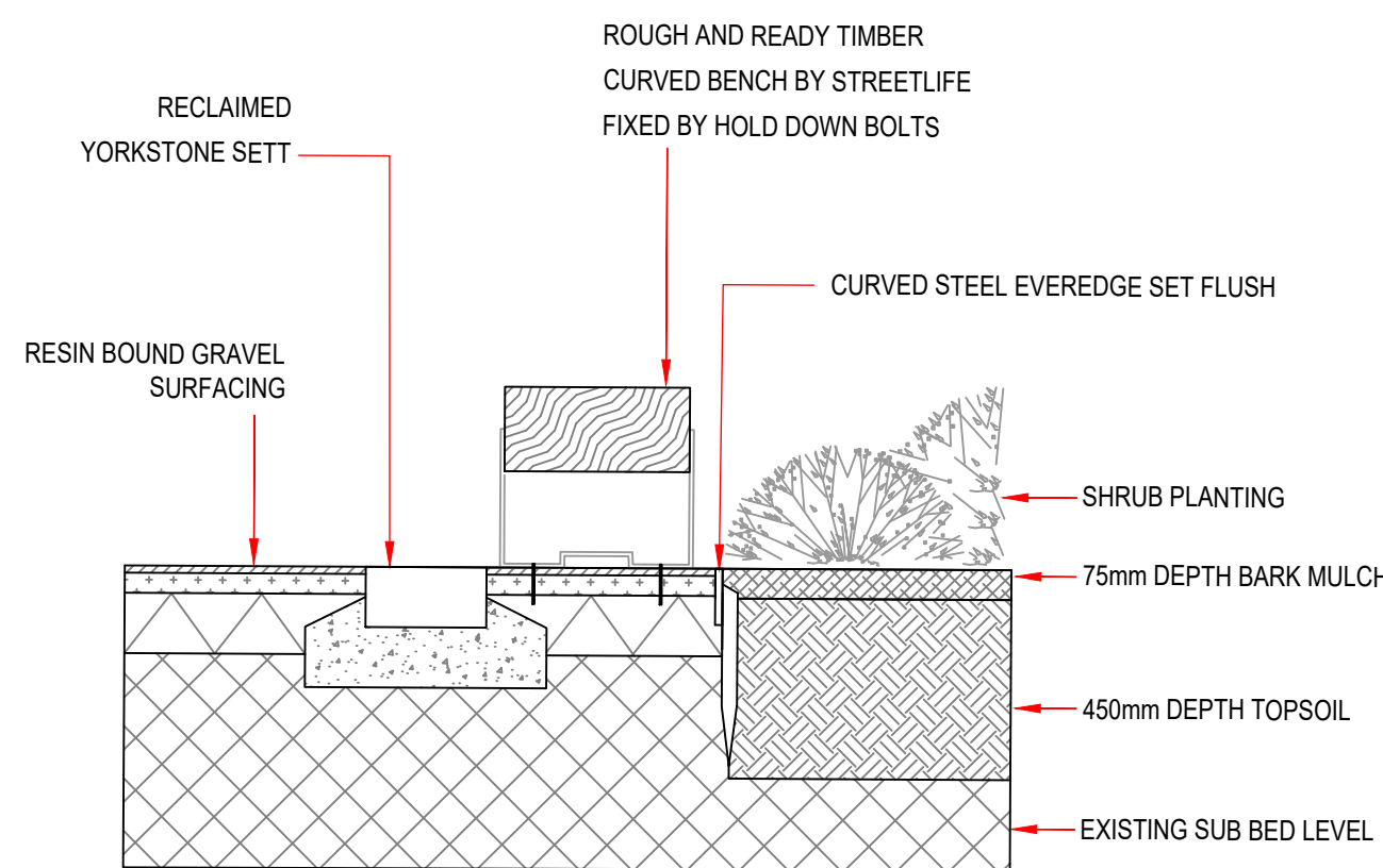
17 1:20 CURVED BENCH ADJACENT TO SHRUB PLANTING
