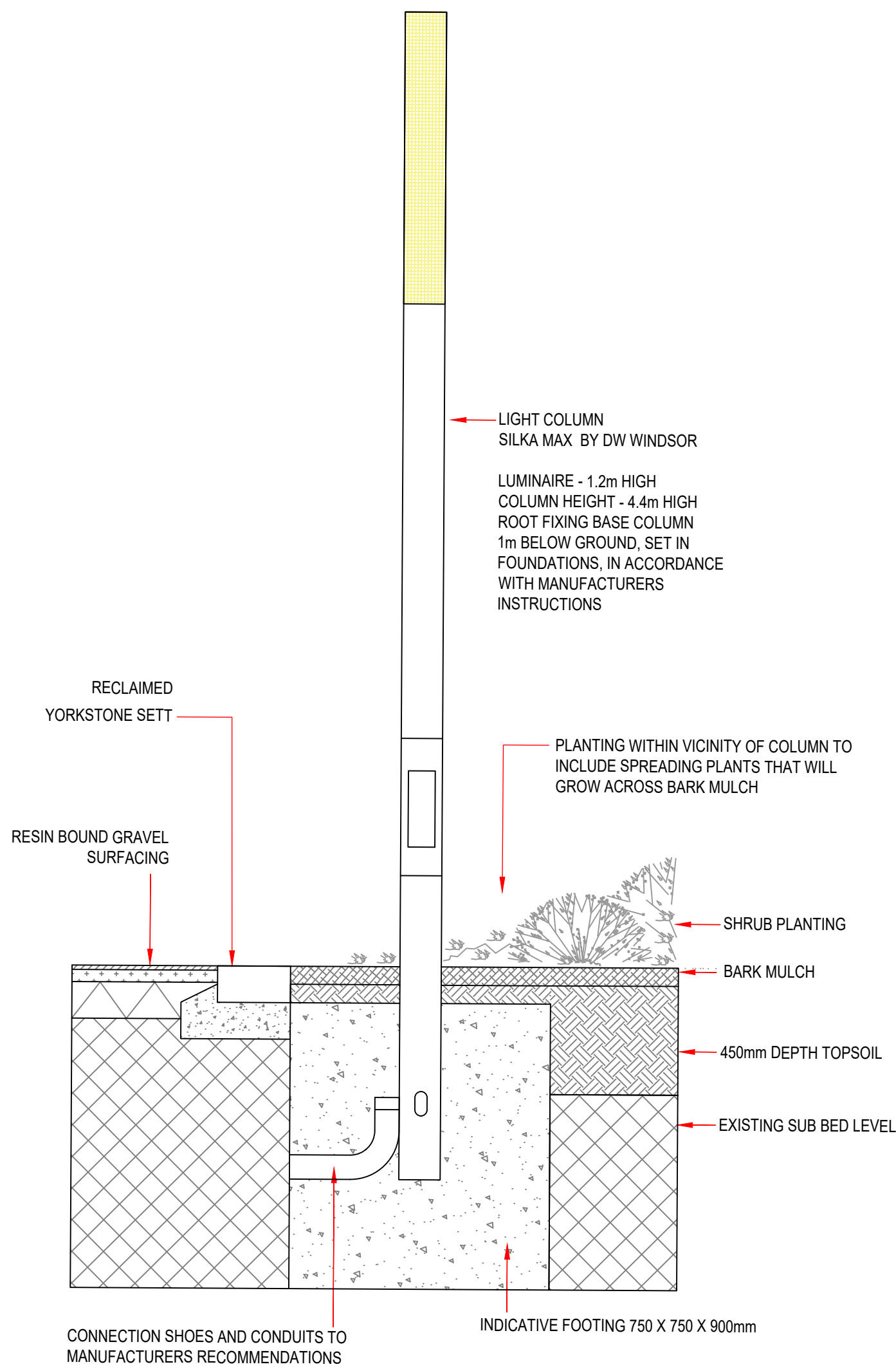
16 1:20 SILKA MAX LIGHT COLUMN SET INTO SOFT LANDSCAPE
