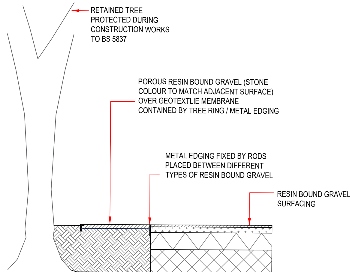
18 1:20 EXISTING TREE RETAINED WITH NEW RECESSED TREE GRILLE, INFILLED WITH RESIN BOUND GRAVEL
