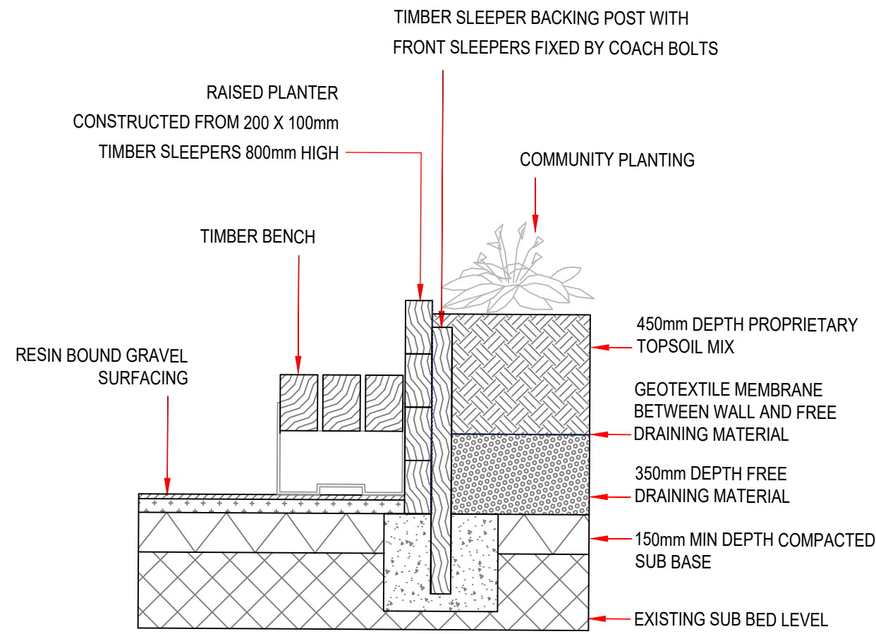
12 1:20 RAISED TIMBER PLANTER WITH INTEGRATED SEATING
