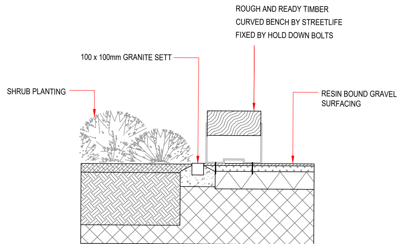
15 1:20 TIMBER BENCH ADJACENT TO SHRUB PLANTING
