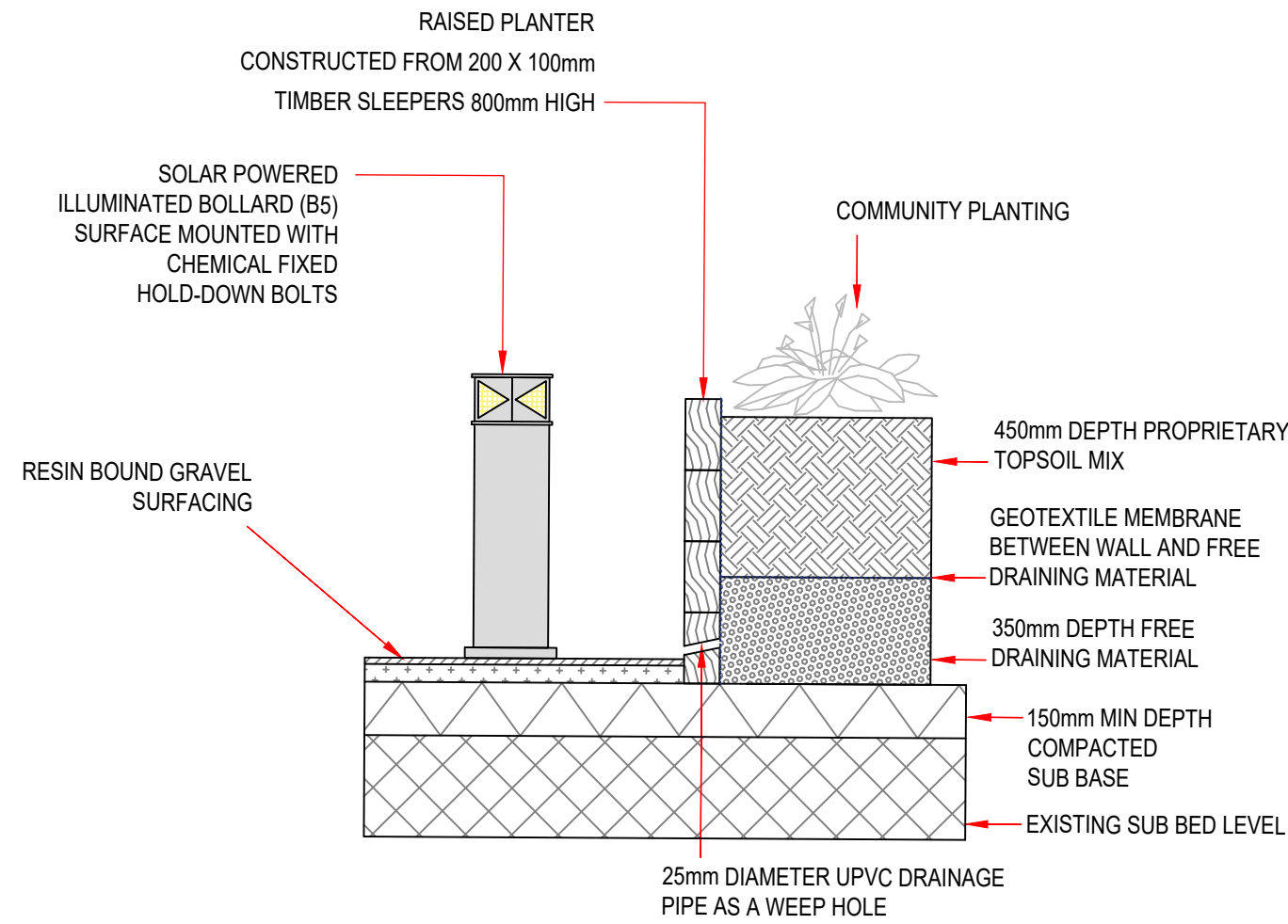
13 1:20 ILLUMINATED BOLLARD ADJACENT TO RAISED TIMBER PLANTER
