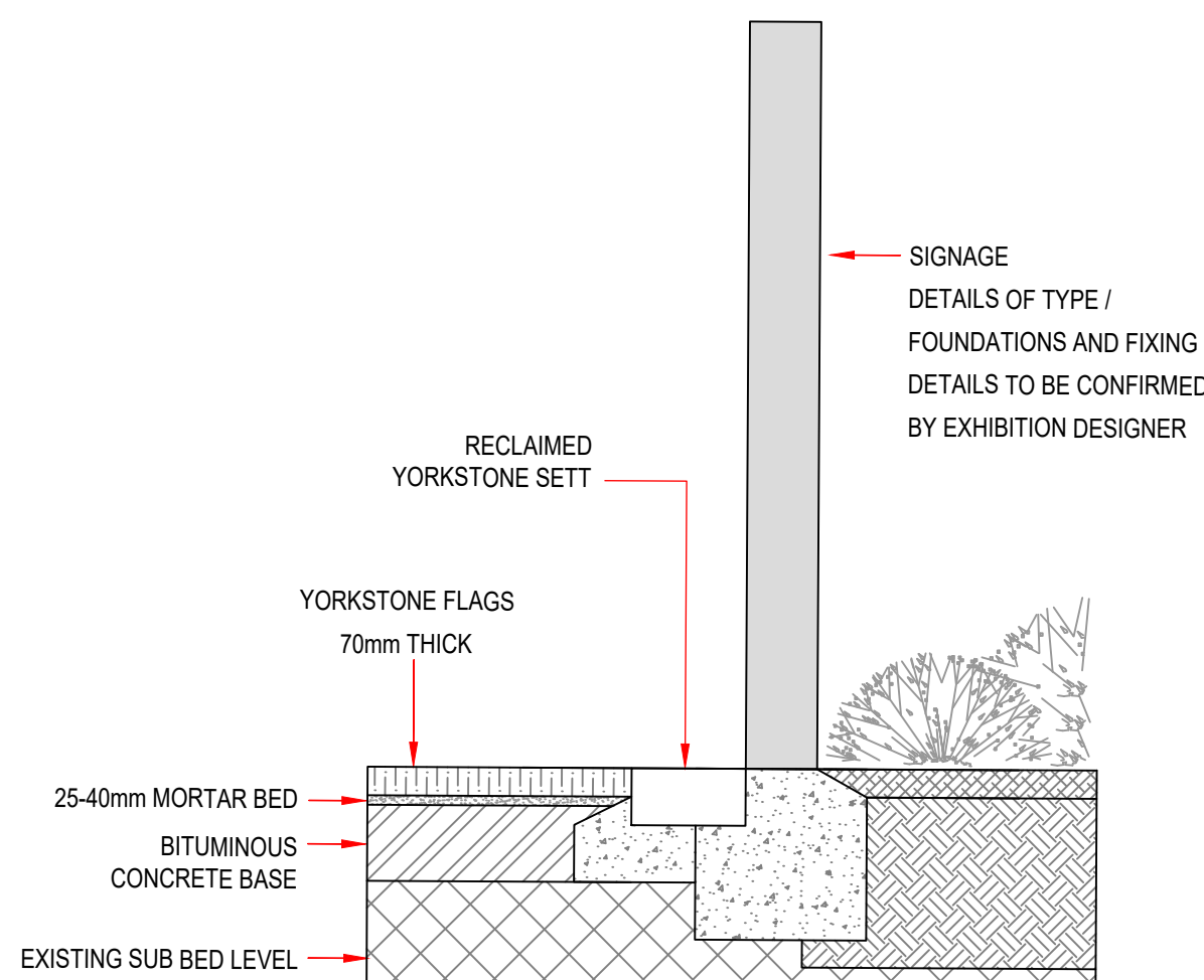
20 1:20 SIGNAGE AT MAIN ENTRANCE
