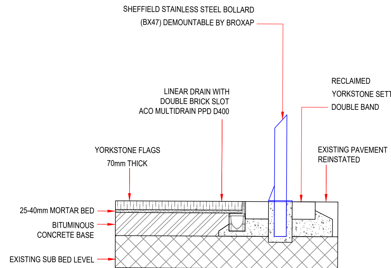
21 1:20 LINEAR DRAIN WITH DOUBLE BRICK SLOT / DEMOUNTABLE STAINLESS STEEL BOLLARD
