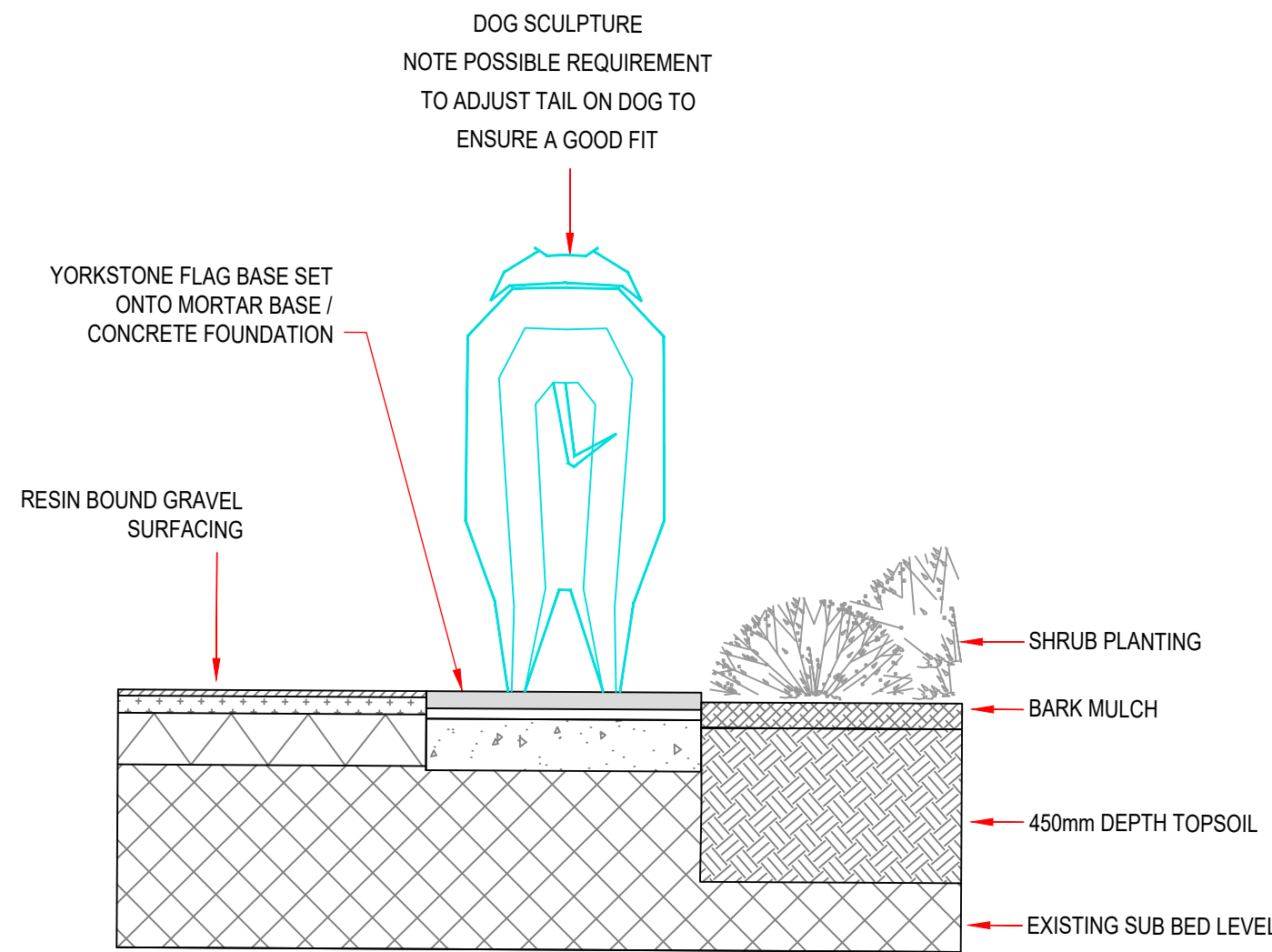
14 1:20 DOG SCULPTURE - RELOCATED FROM ENTRANCE
