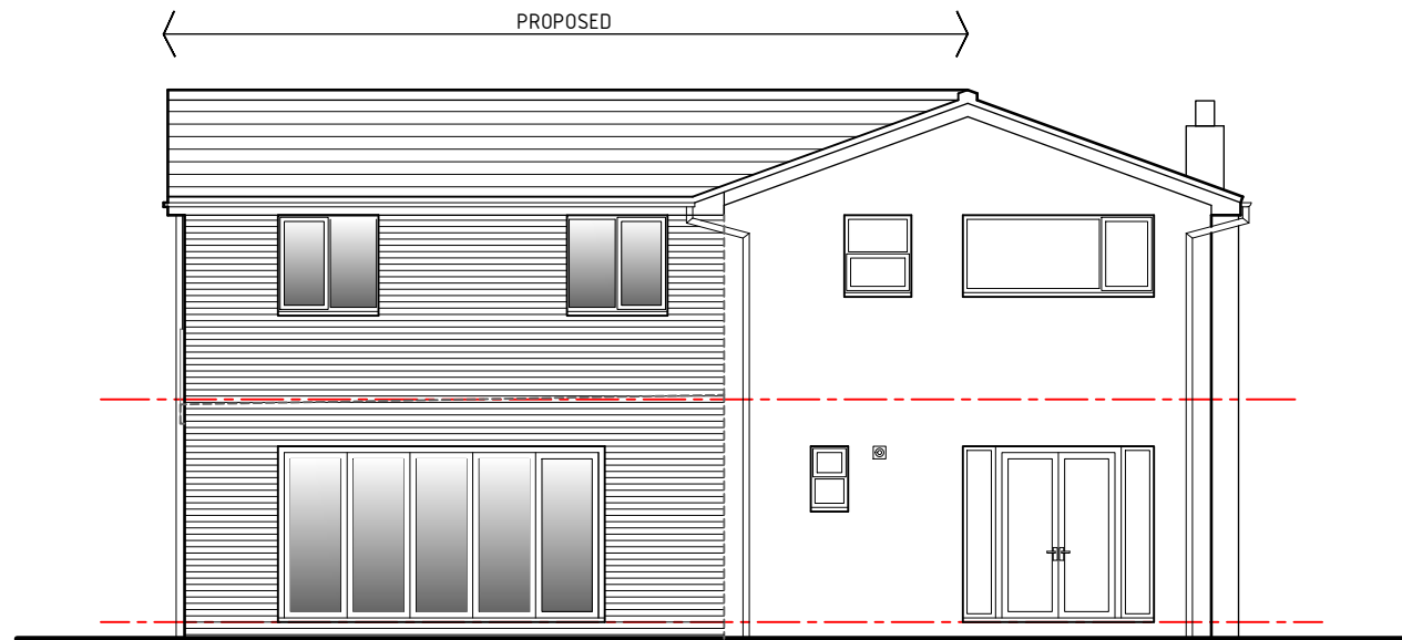
Rear elevation 1:100
