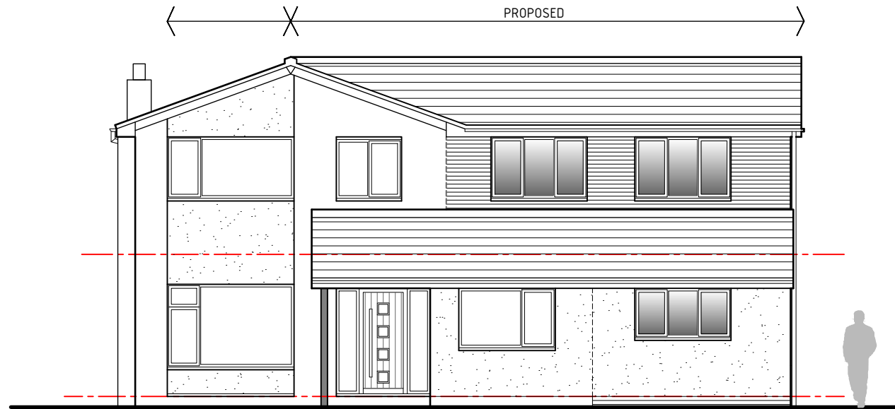
Front elevation 1:100
