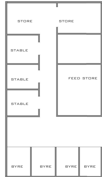
A 7 1:100 Floor Plan
