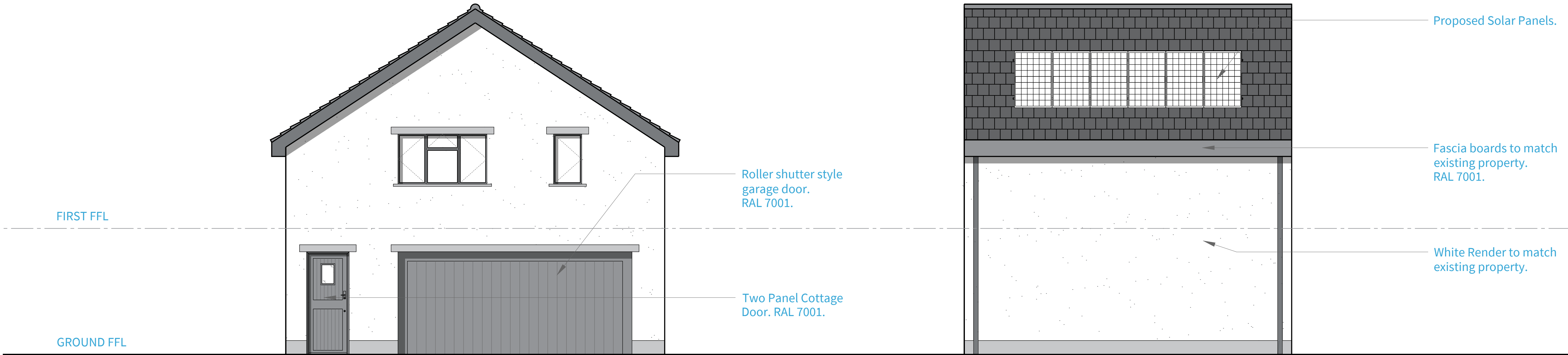
ELEVATION A SCALE 1:50
