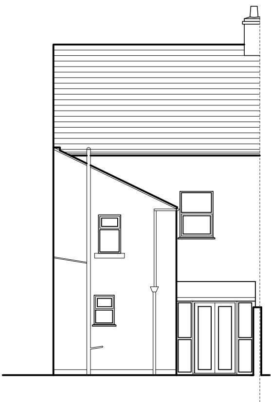
2 REAR ELEVATION
