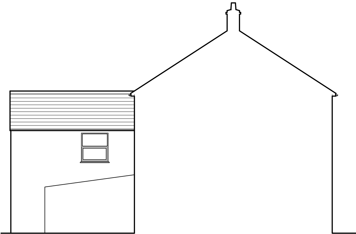
1 SIDE ELEVATION
