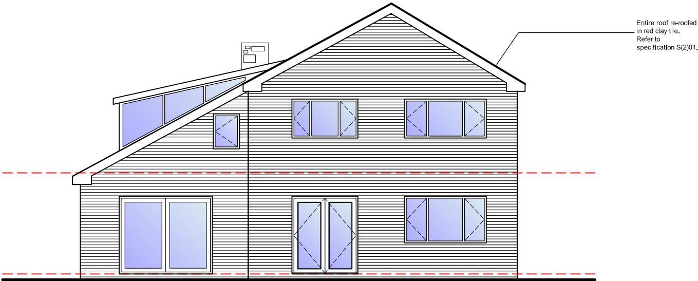
REAR ELEVATION
