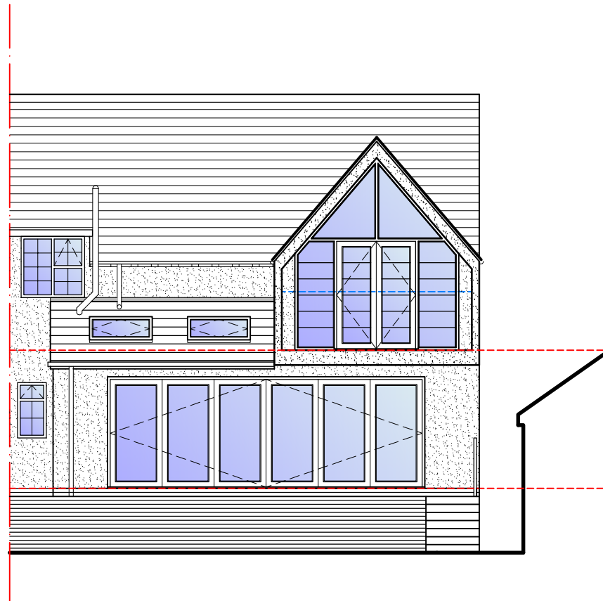
REAR ELEVATION
