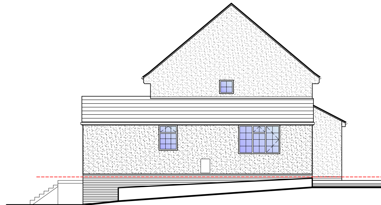
SIDE ELEVATION
