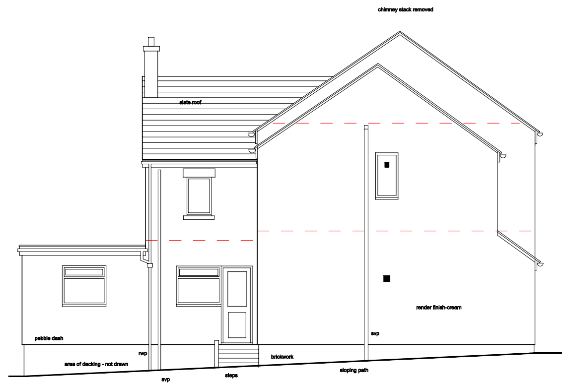
WEST ELEVATION GABLE
