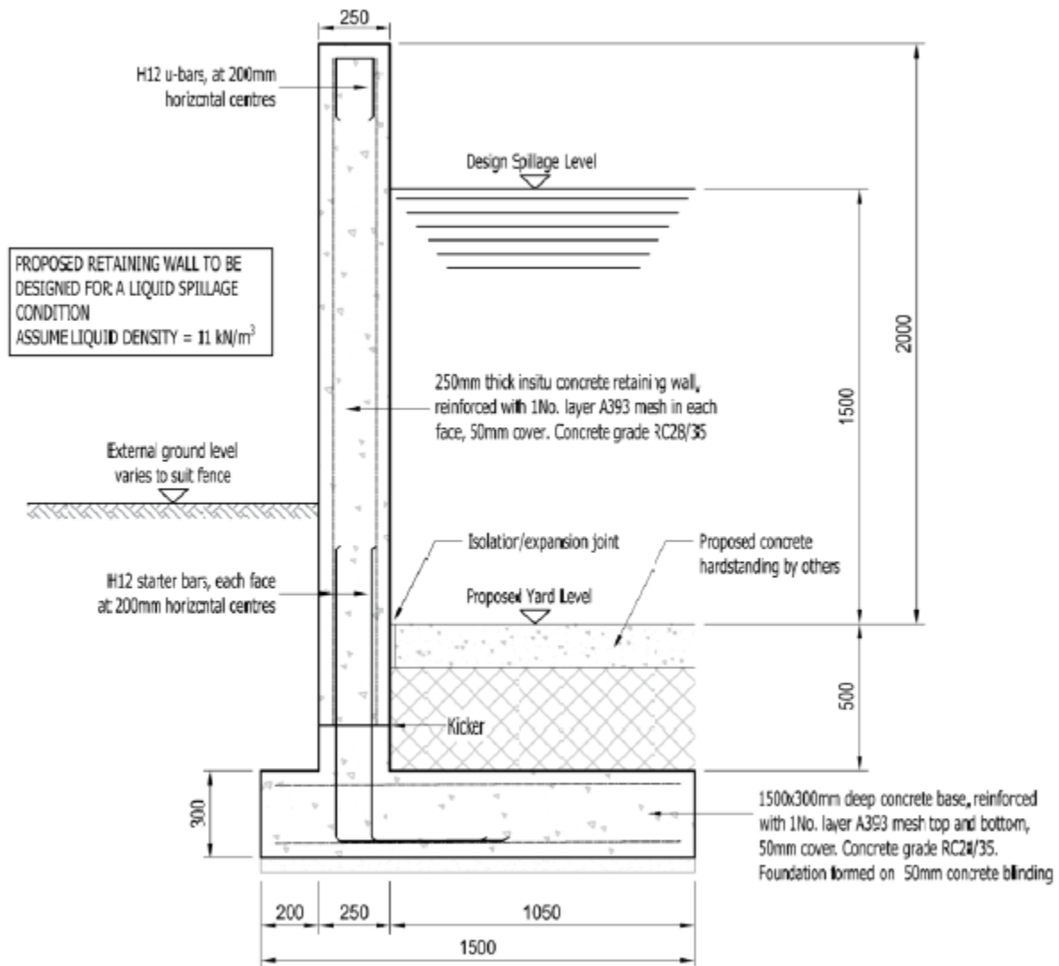
RETAINING WALL 1
