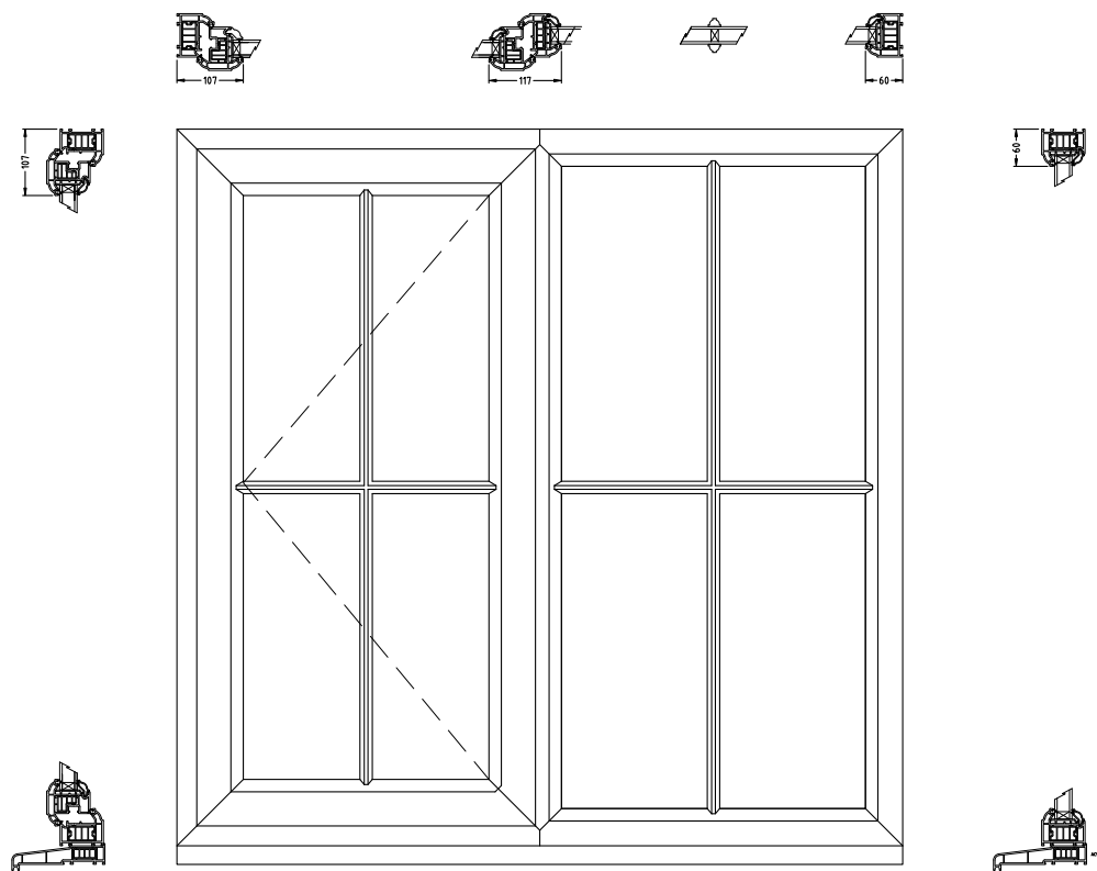
15 WHITEGATE FIELDS TYPICAL PROPOSED WINDOW ELEVATION AND SECTIONS
