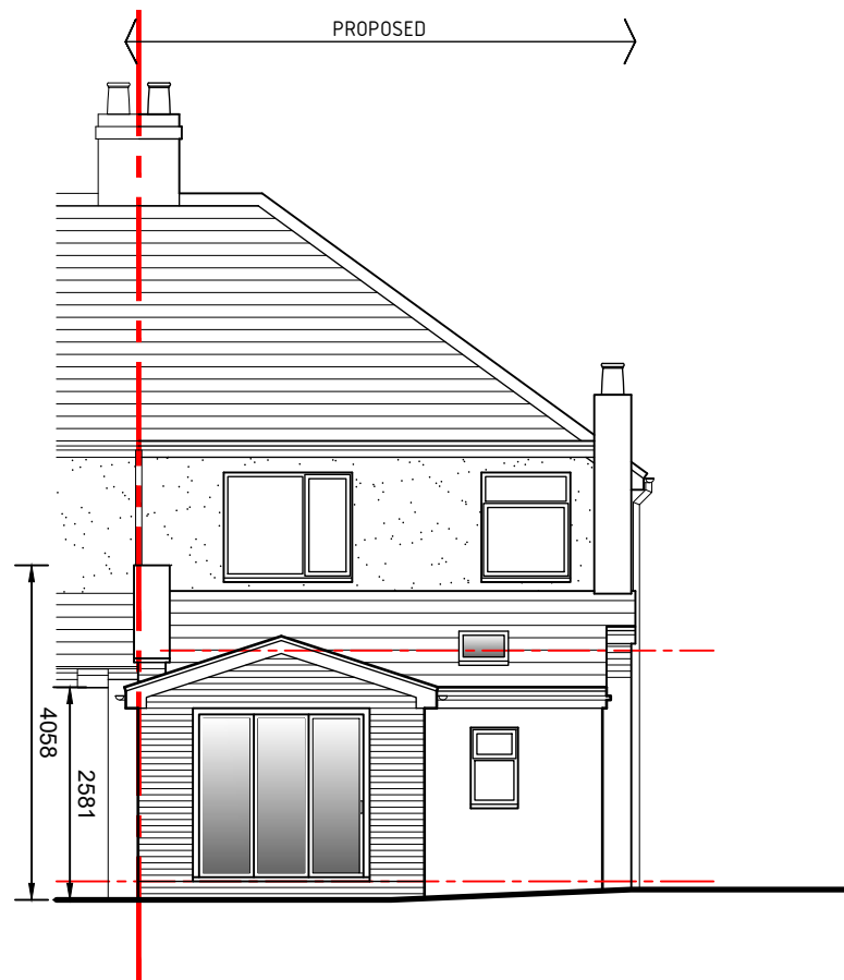
Rear elevation 1:100
