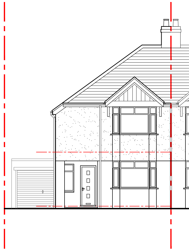
Front elevation 1:100
