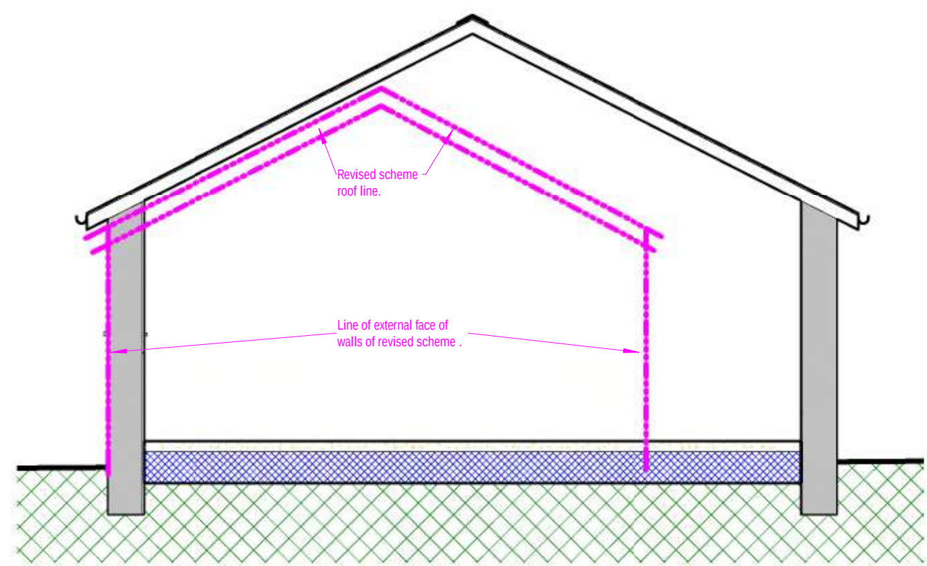
GENERAL SECTION
