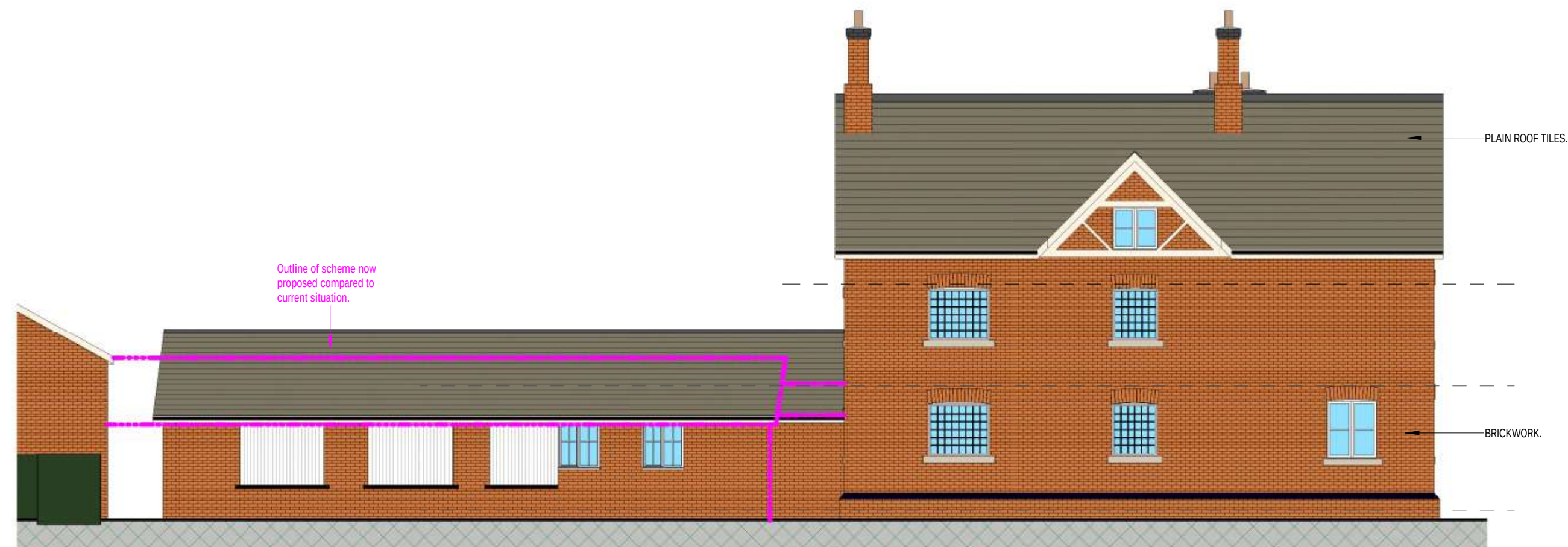
FRONT ELEVATION.
