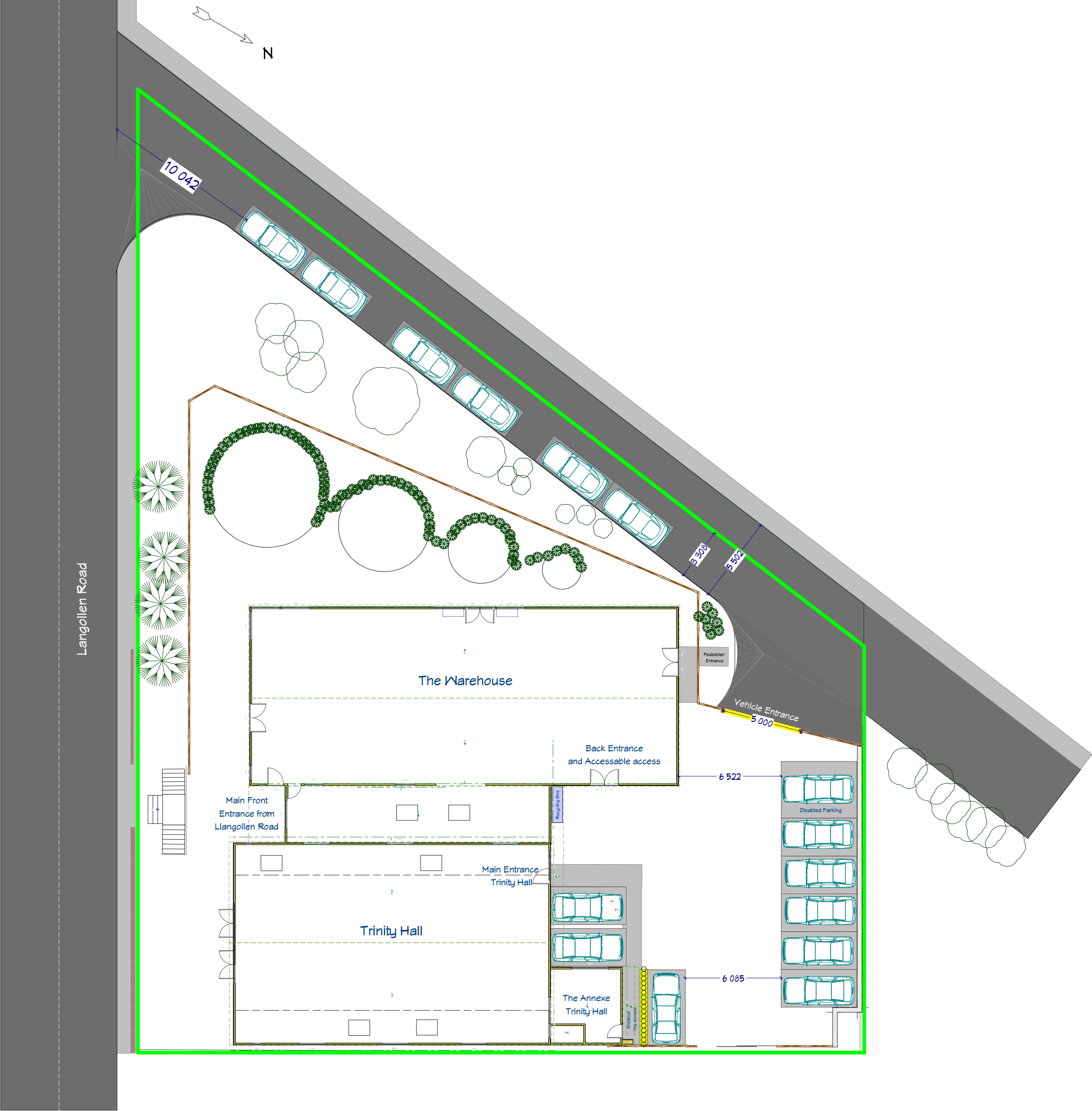
DIAGRAM A - Trinity Hall - To Scale Site plan
