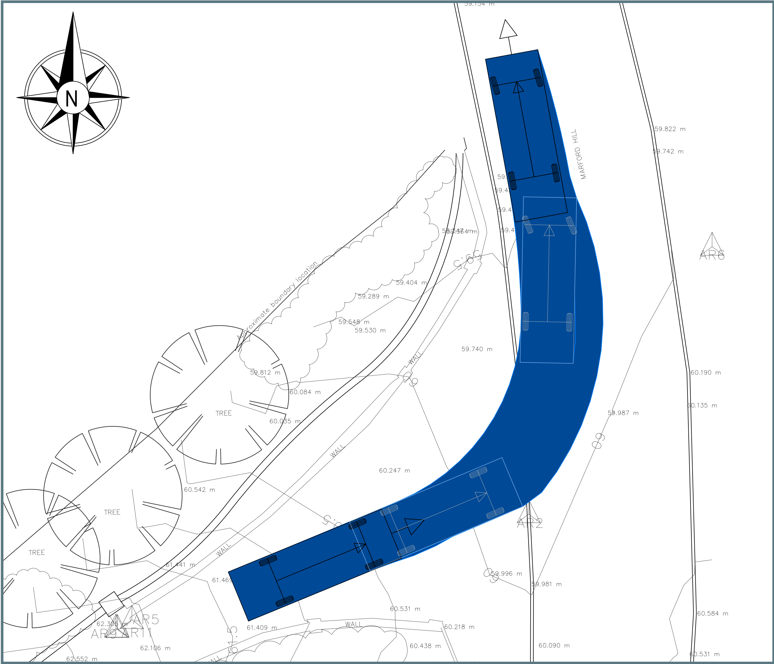
LEFT TURN LG RIGID VEHICLE SCALE: 1:100
