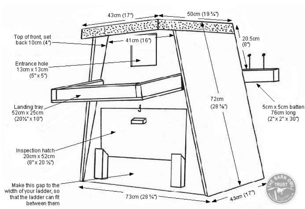
FIGURE 5.3: BARN OWL NEST BOX DESIGN FOR EXTERIOR USE
