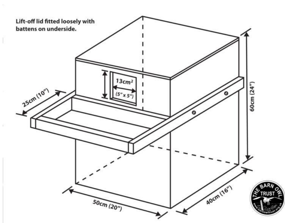
FIGURE 5.2: BARN OWL NEST BOX DESIGN FOR USE INSIDE BUILDINGS
