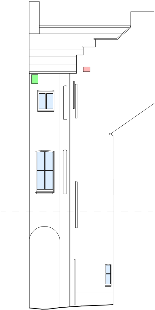
REAR ELEVATION
