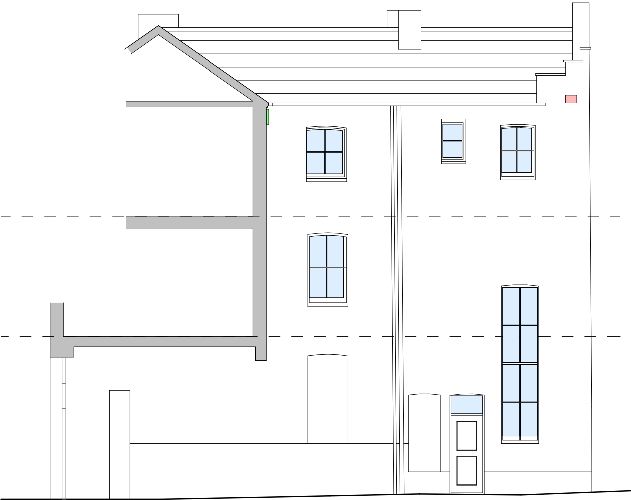
SIDE ELEVATION
