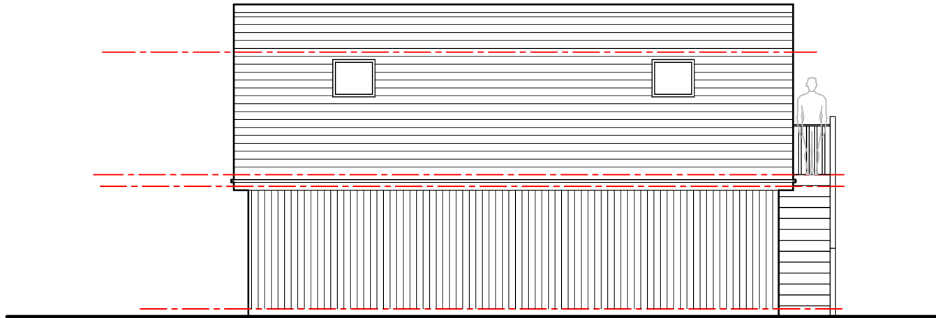
Rear Elevation 1:100
