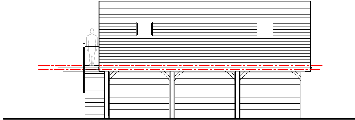
Front Elevation 1:100
