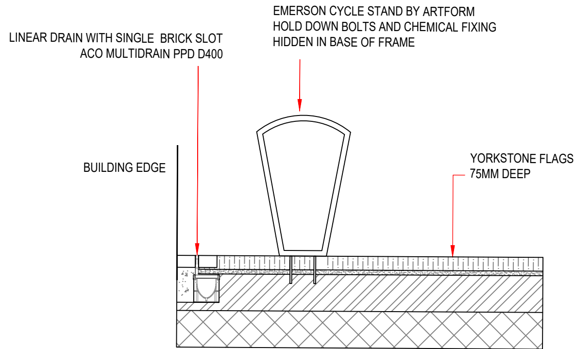
25 1:20 BARRIER AND SLOT DRAIN ADJACENT TO BUILDING EDGE
