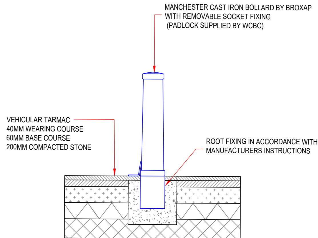
28 1:20 DEMOUNTABLE CAST IRON BOLLARD TO SIDE ENTRANCE
