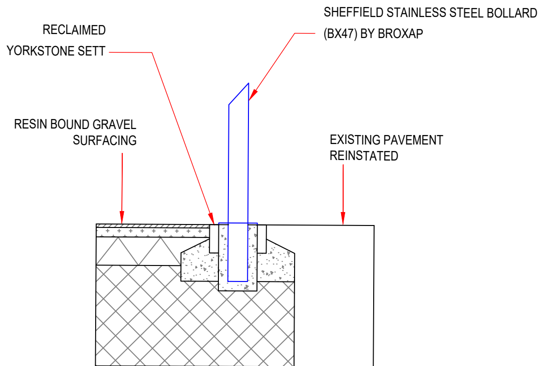
24 1:20 STAINLESS STEEL BOLLARD SET IN RECLAIMED YORKSTONE BANDING
