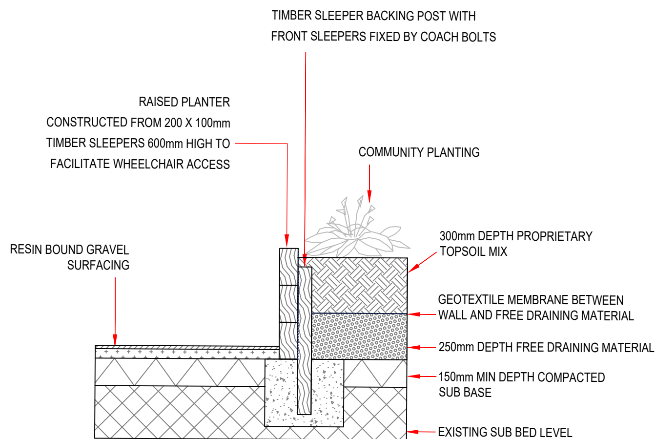
30 1:20 SECTION OF RAISED PLANTER LOWERED TO FACILITATE WHEELCHAIR ACCESS
