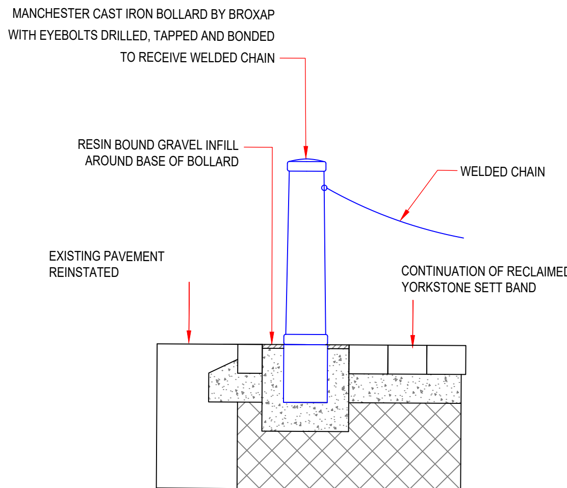
29 1:20 FIXED CAST IRON BOLLARD TO SIDE ENTRANCE WITH CHAIN FIXINGS
