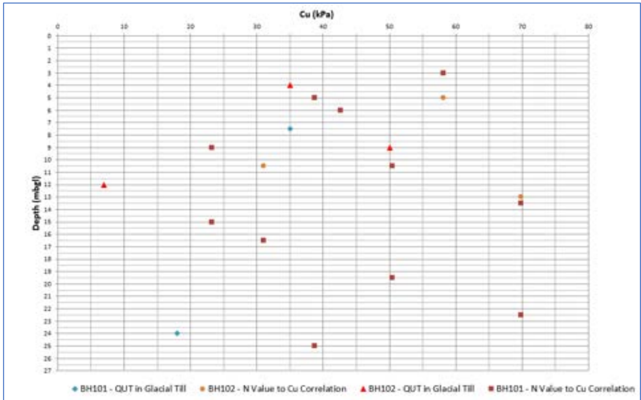
Figure 17. Glacial Till – C_u from QUT and SPT N Value Correlations
