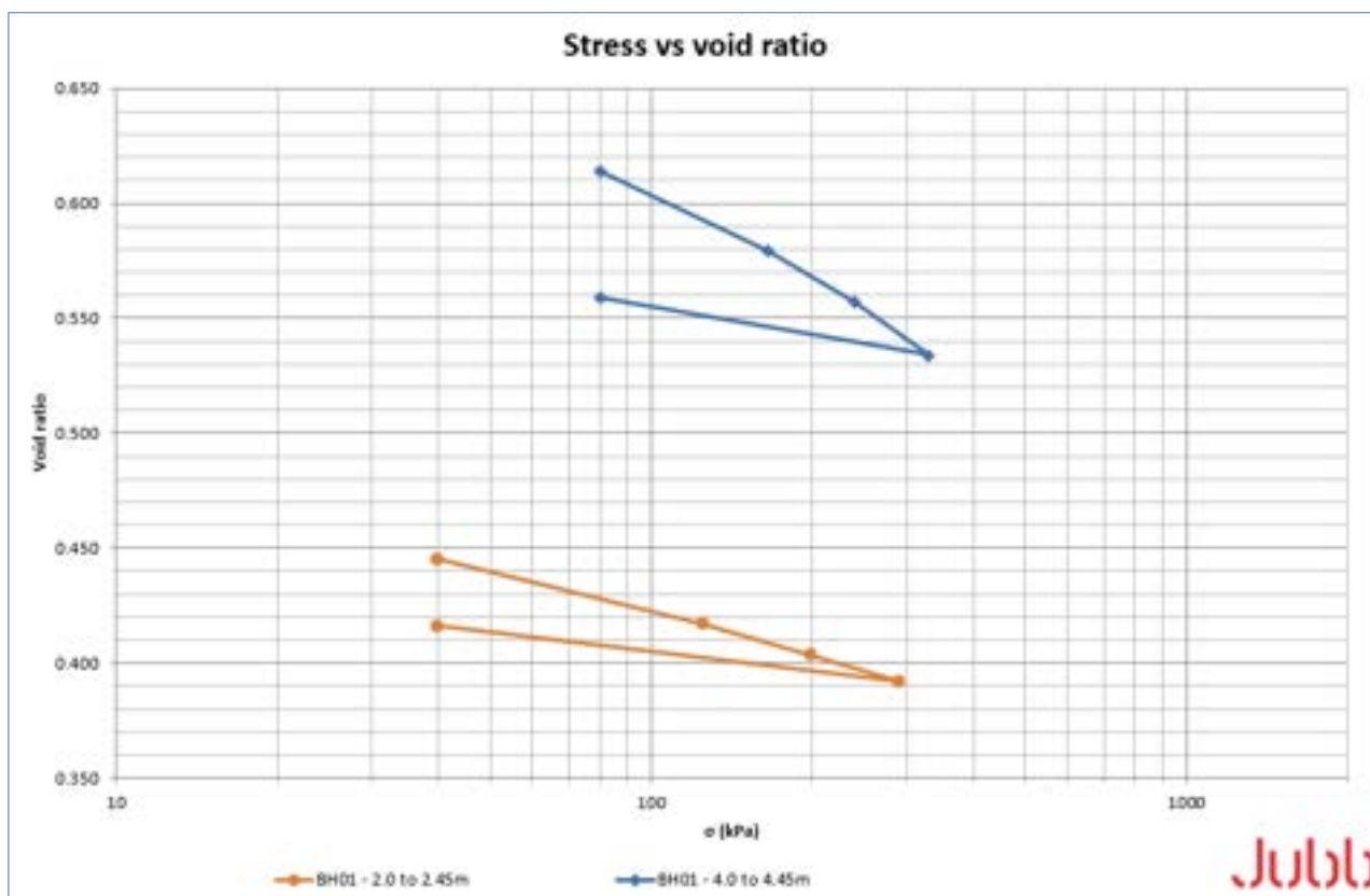
Figure 18: Oedometer Test Results - Glacial Till
