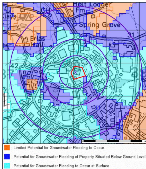
Figure 6: BGS Groundwater Flooding Susceptibility Map (Site location in red)
