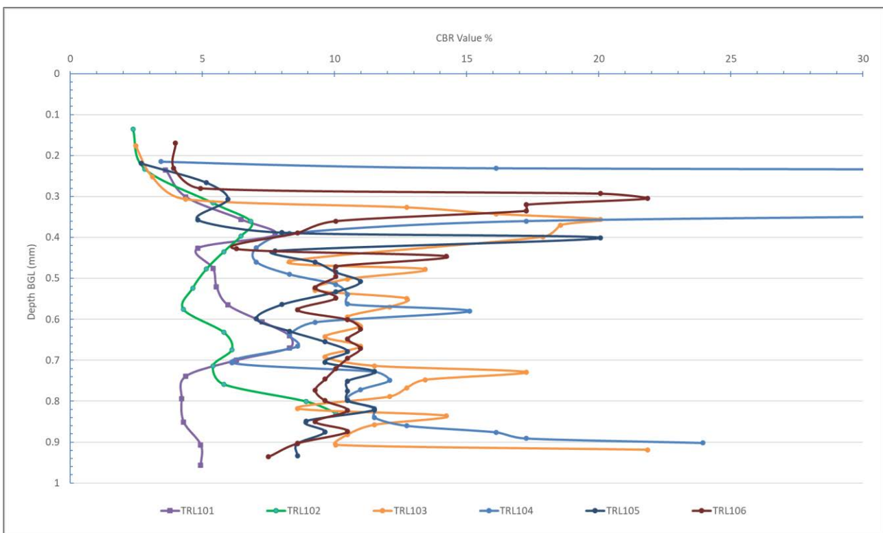
Figure 19: CBR vs Depth correlated from DCP testing
