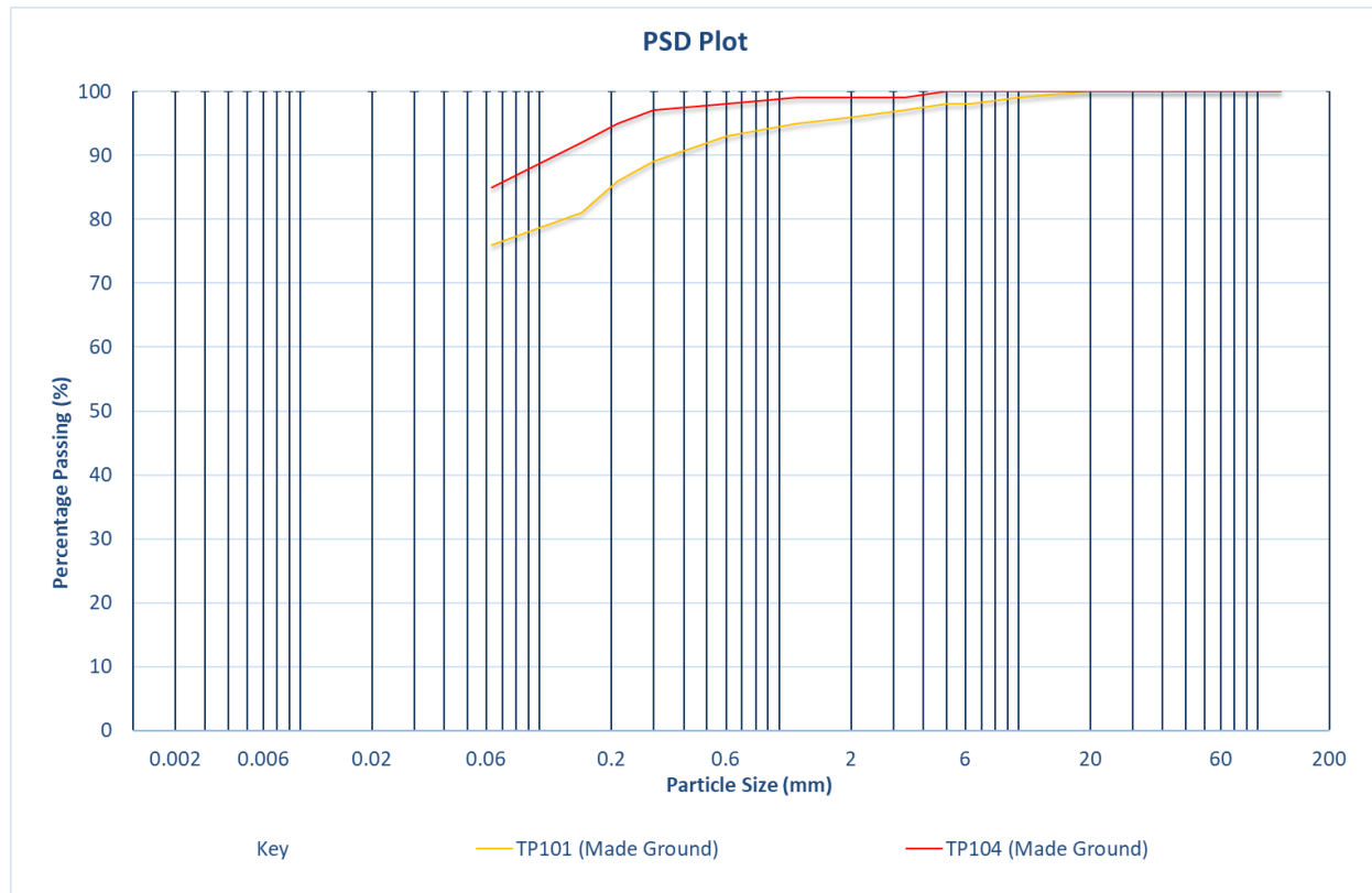
Figure 10: Particle size distribution chart of Made Ground
