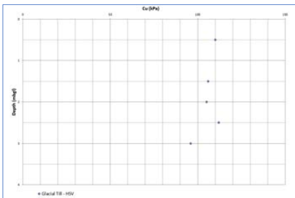
Figure 16: HSV Values for Glacial Till
