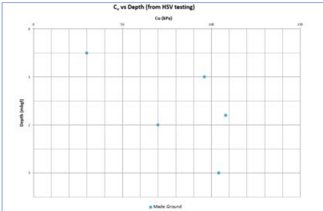
Figure 11. Made Ground - Hand Shear Vane results.
