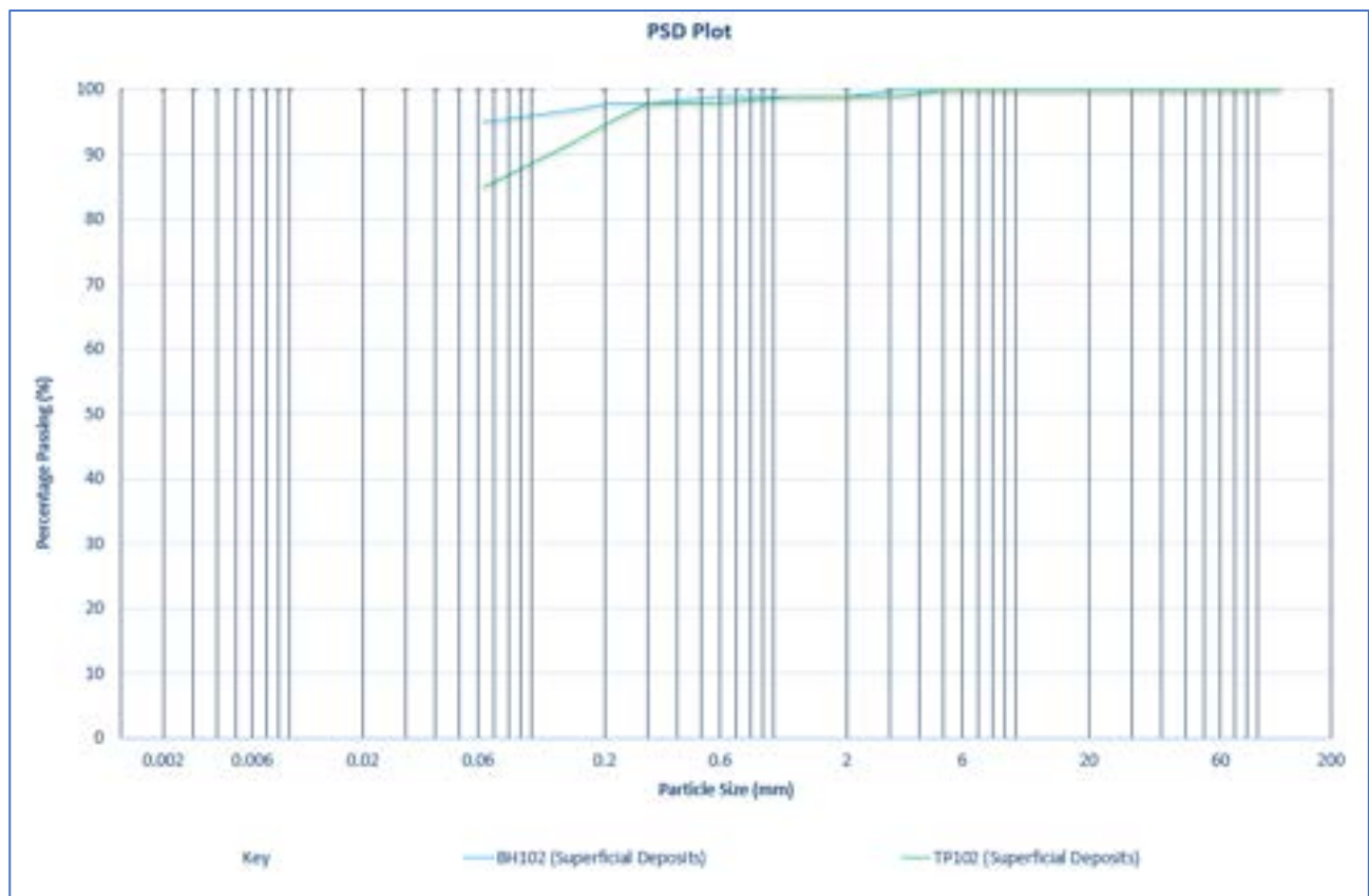
Figure 14: Particle size distribution chart of Glacial Deposits
