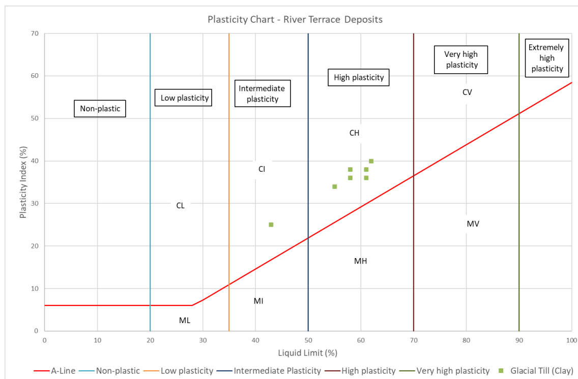
Figure 13: Glacial Deposits Atterberg Testing
