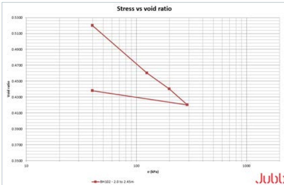
Figure 12: Made Ground Oedometer results
