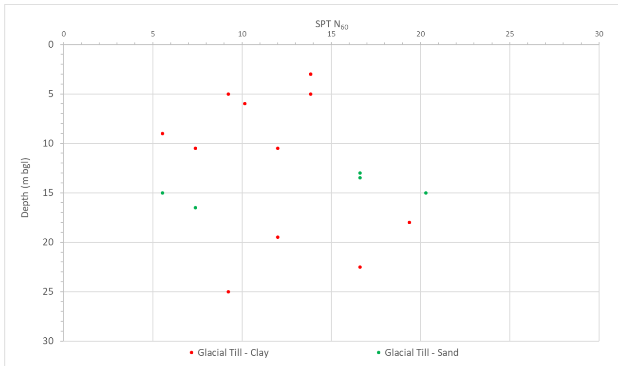
Figure 15. SPT Results – Glacial Deposits
