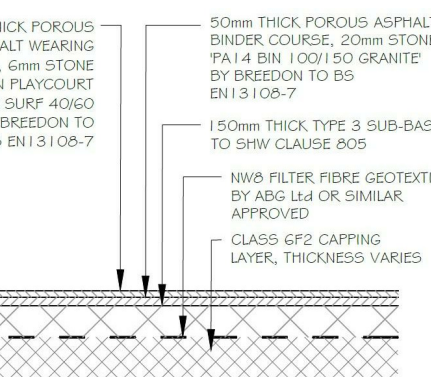
Asphalt Footway Indicative detail Final construction details to be agreed with Structural Engineer
