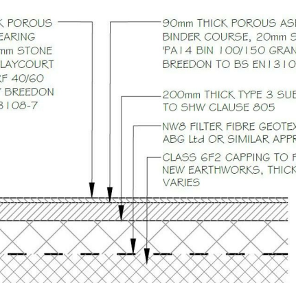
Asphalt Carriageway (parking & crossovers) Indicative detail Final construction details to be agreed with Structural Engineer
