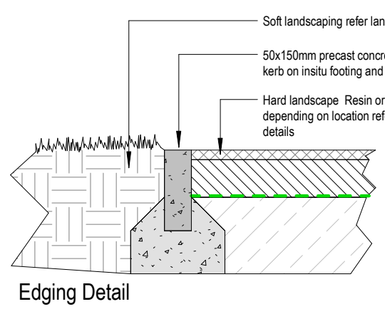
Edging Detail
