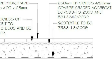
Paved Footway Indicative detail Final construction details to be agreed with Structural Engineer
