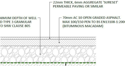
Resin Bound Gravel Footway Indicative detail Final construction details to be agreed with Structural Engineer
