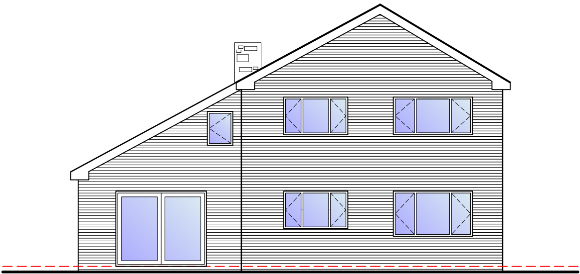
REAR ELEVATION
