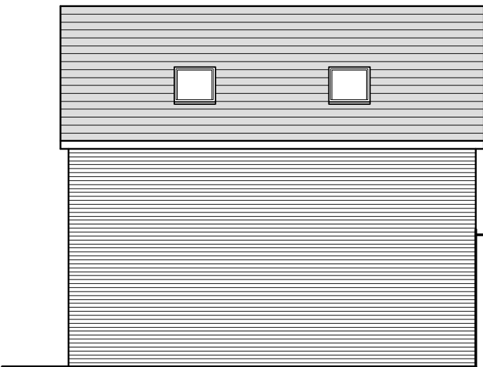
Side Elevation 1:100
