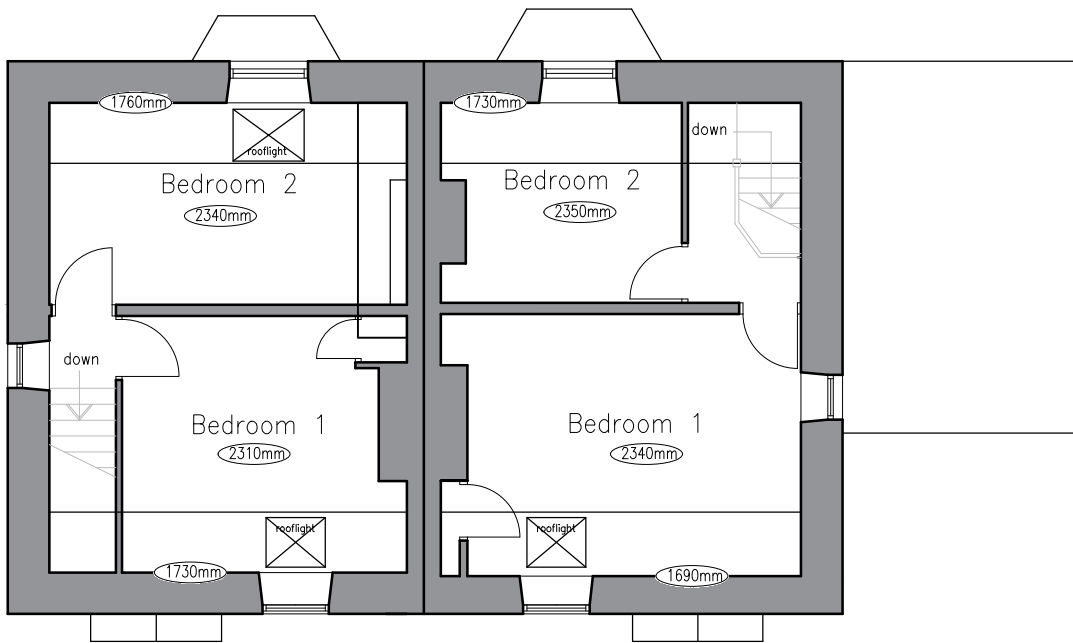
NO.2 NANTYR ROAD NO.3 NANTYR ROAD EXISTING FIRST FLOOR PLAN
