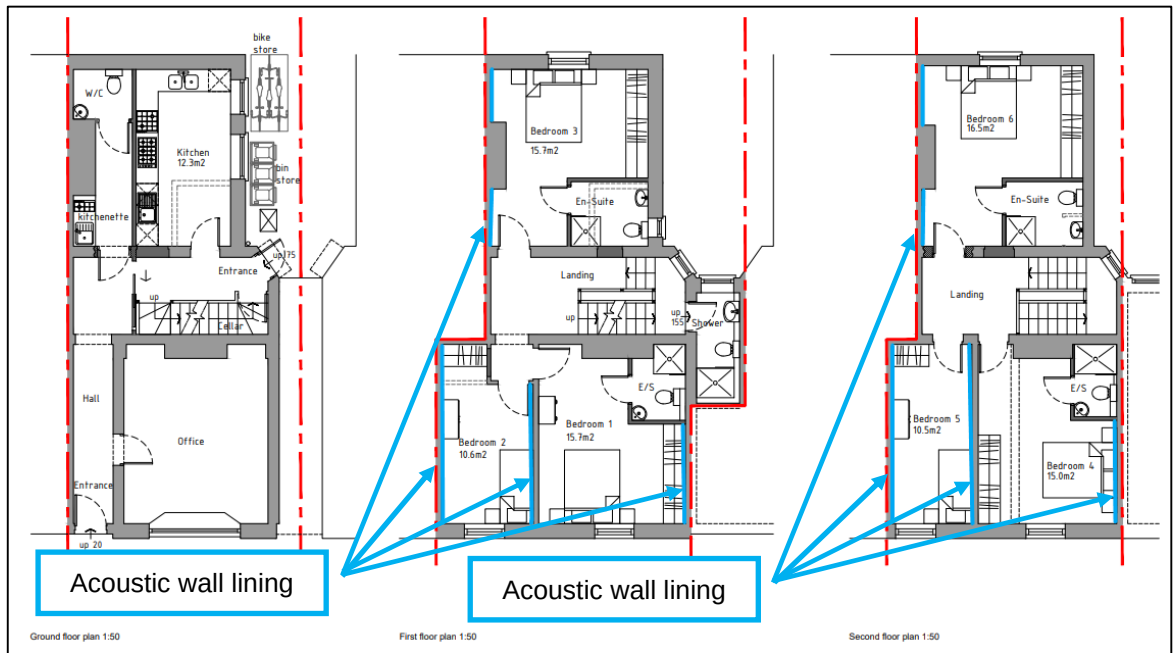
Figure 4.4 - Floor layouts showing independent wall linings
