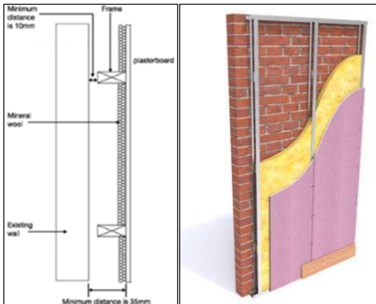
Figure 4.3 - Diagram showing independent wall lining
