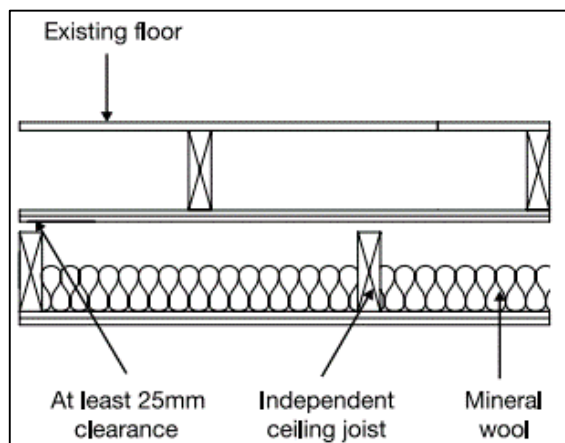
Figure 4.2 - Diagram showing independent timber frame/joists
