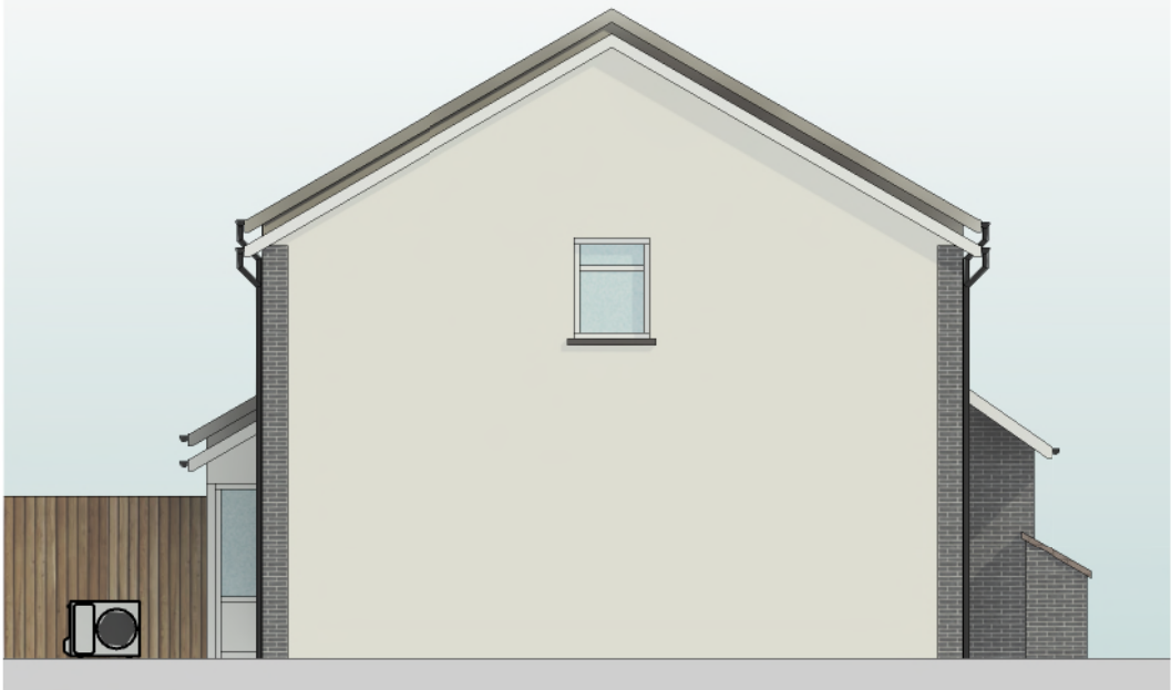
2 East Elevation
