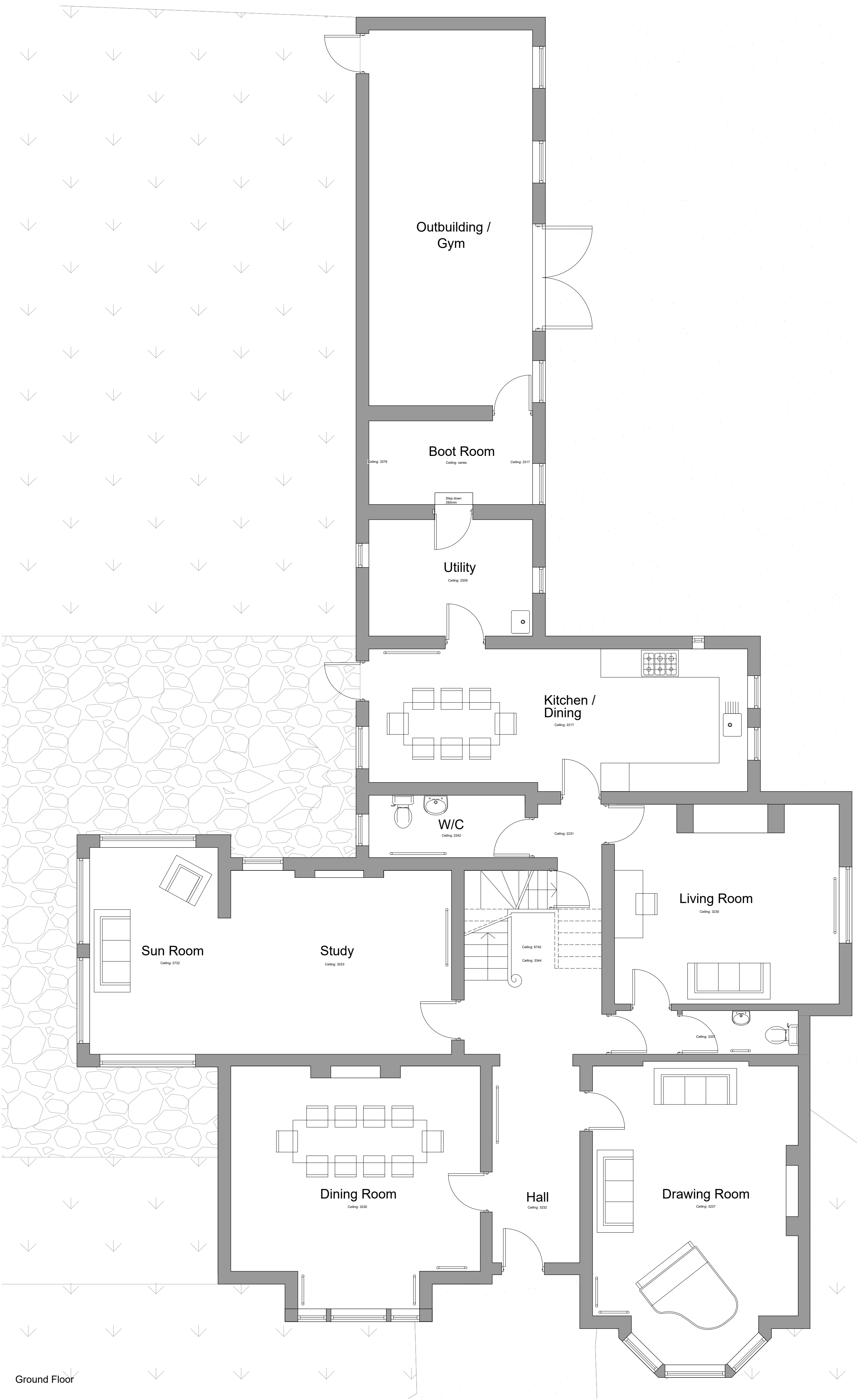
First Floor
