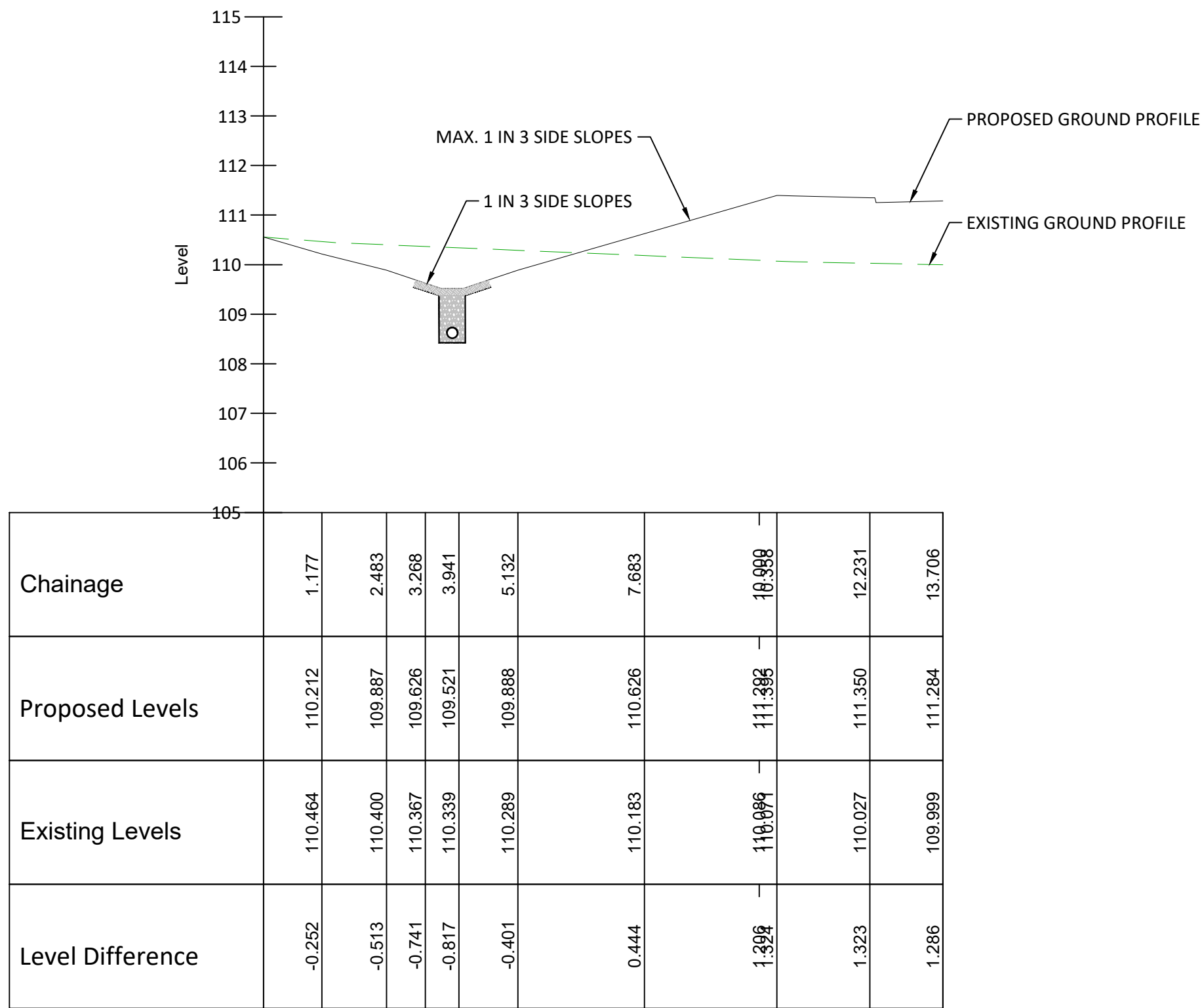
SECTION B-B 1:100
