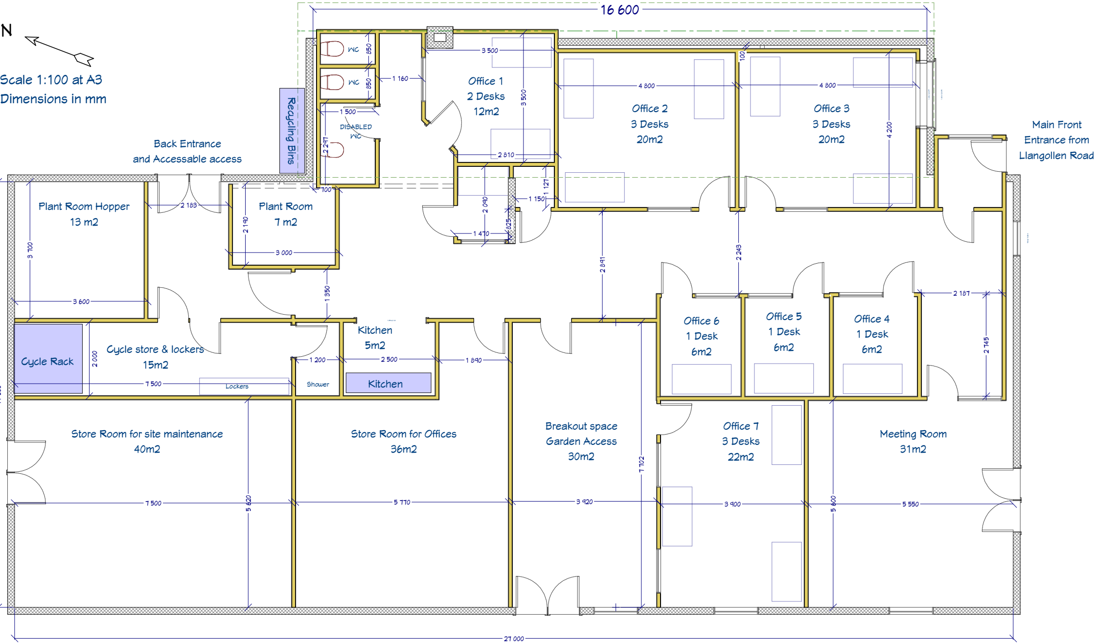
Diagram F - The Warehouse - Proposed Floor plan
