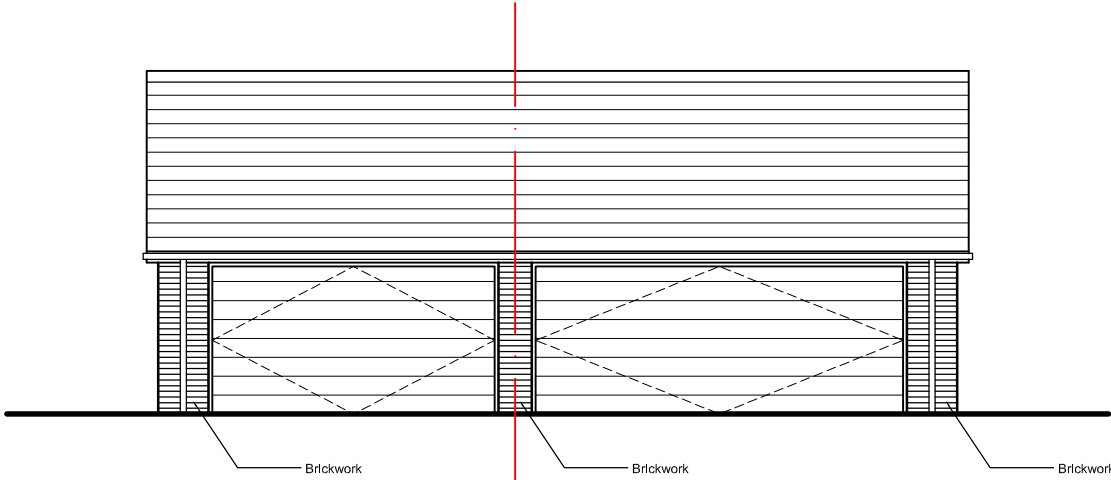
FRONT ELEVATION
