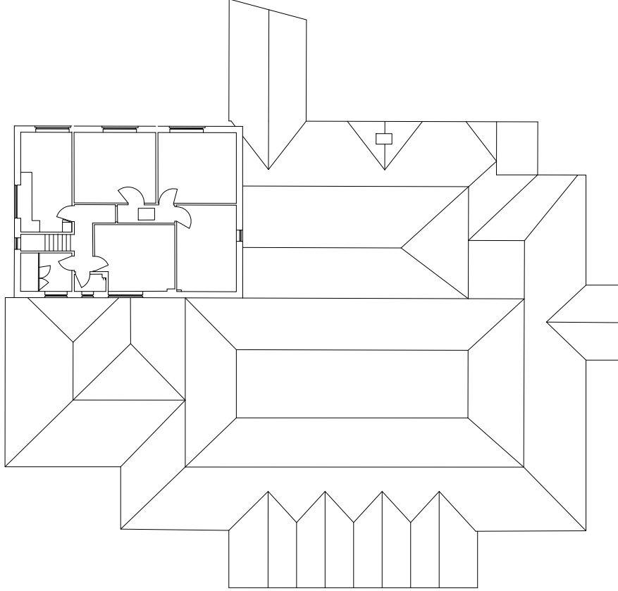
2 EXISTING ROOF PLAN Scale: 1:100
