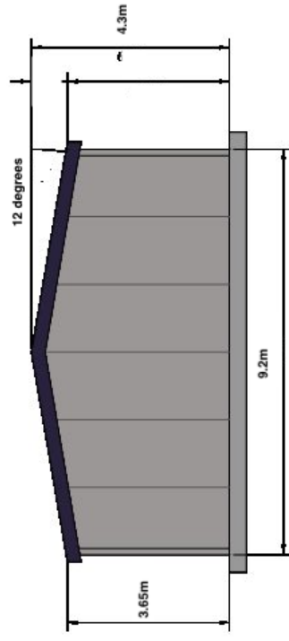
Front Elevation (Exterior)
