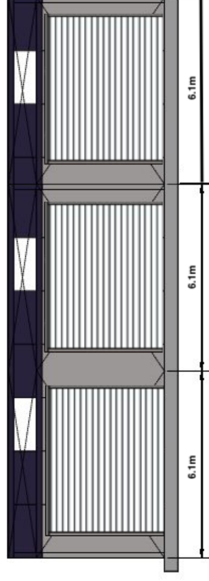
Right Elevation (Scale = 1:100)
