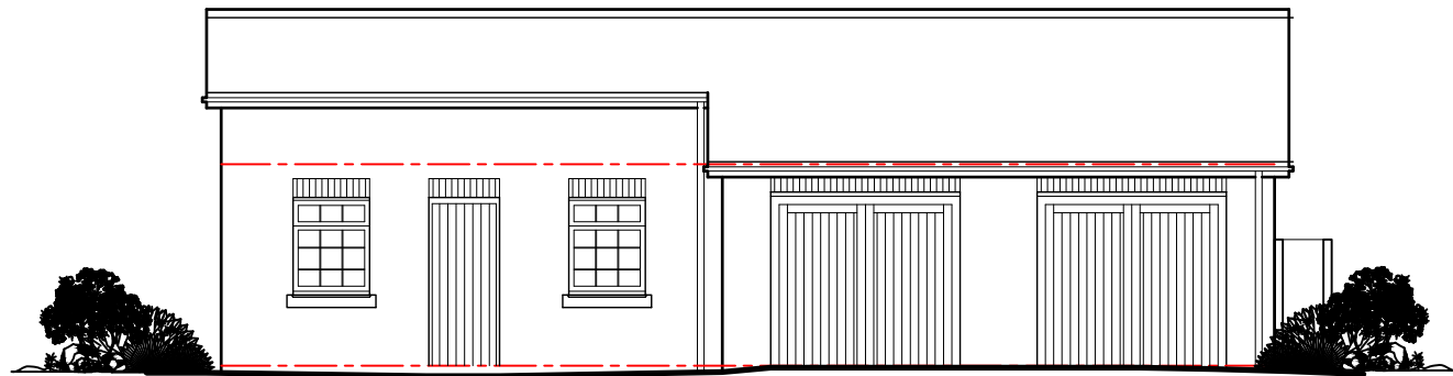
Front elevation 1:100
