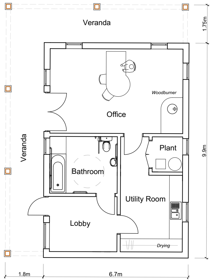
FLOOR PLAN (1/100 @ A2)
