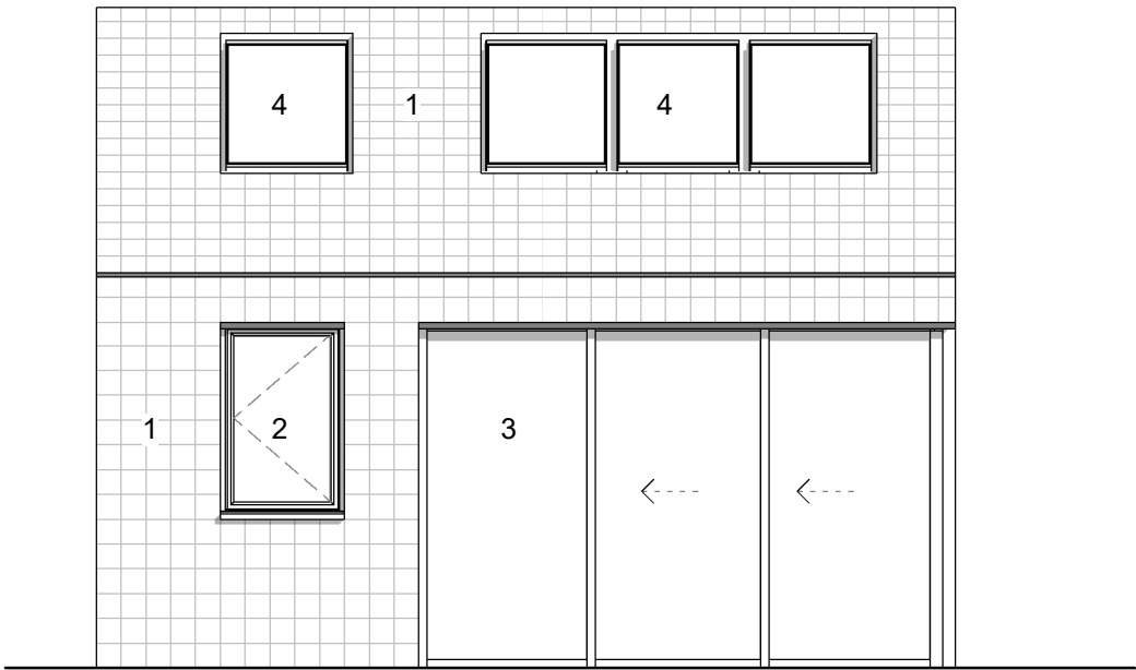
South 1 : 50
