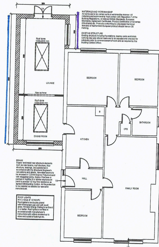
PROPOSED GROUND FLOOR PLAN (scale 1:50)
