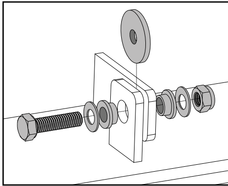
Detail A
