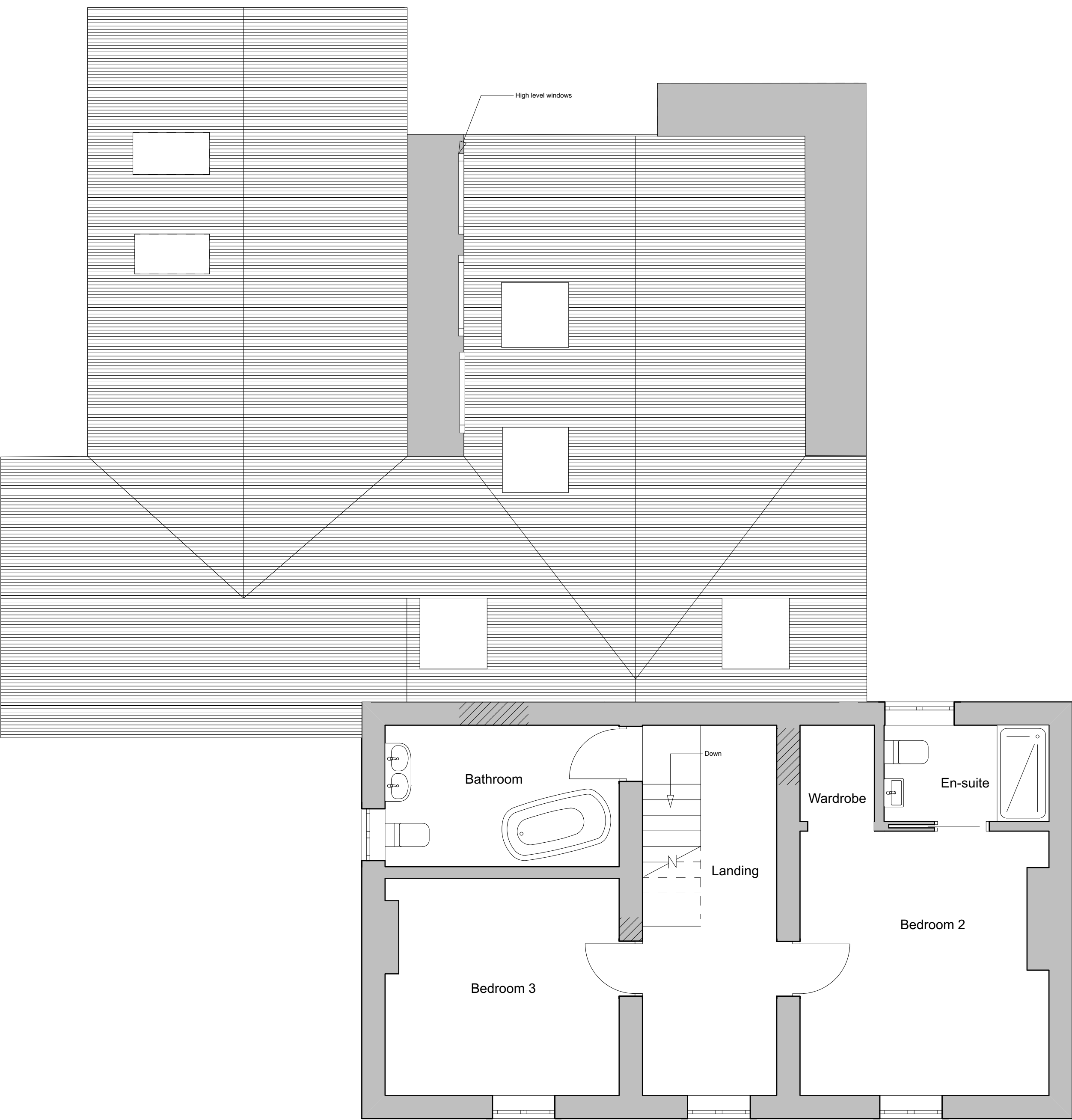
First Floor 1:50
